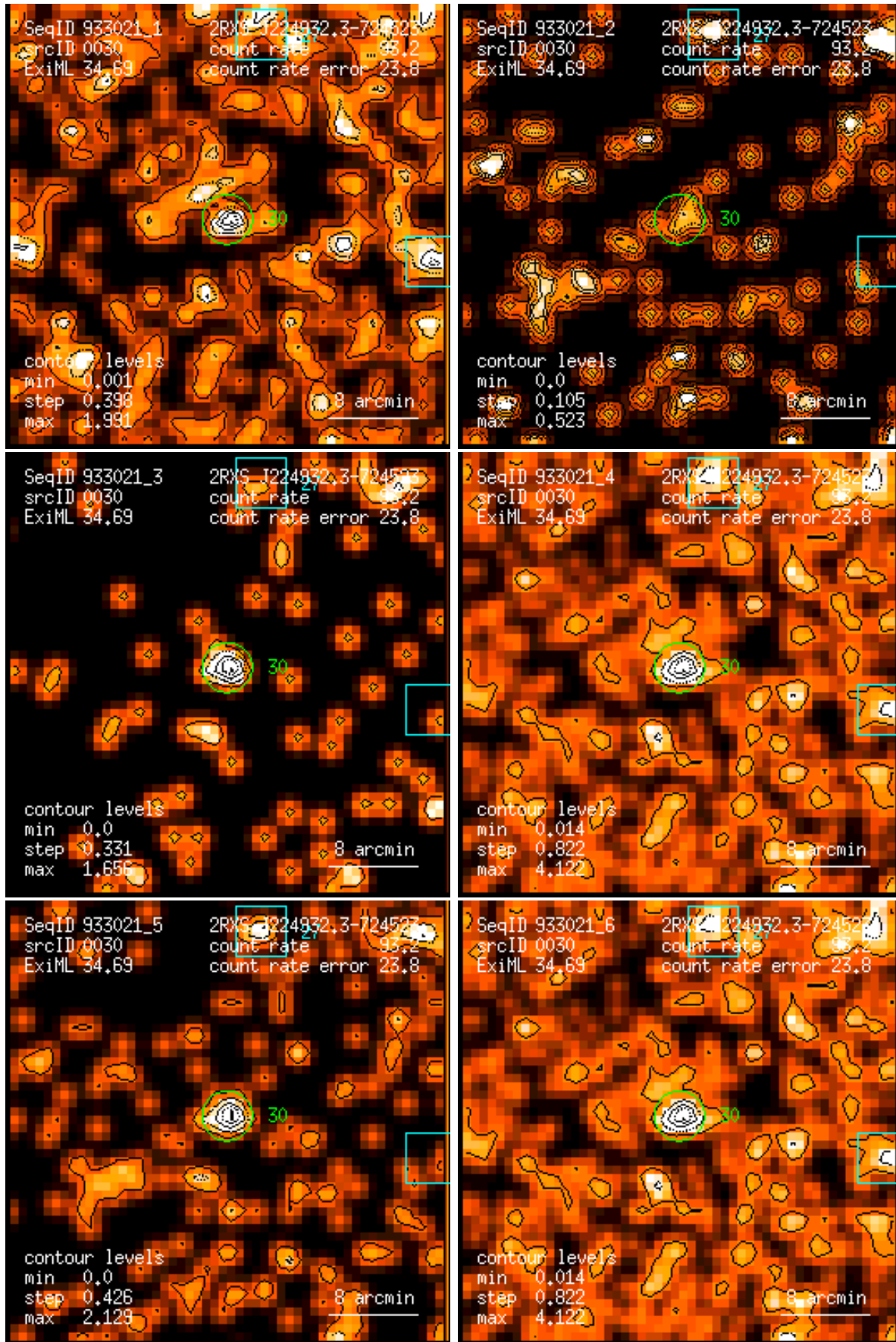
Figure 30: RASS 933021: detection 0030: band rate images, Gaussian filter: (1) PSPC channels 11 – 41, (2) 52 – 90, (3) 91 – 201, (4) 11 – 235, (5) 52 – 201, (6) 11 – 201. Broad band rates in counts/ks. Band rate contour levels in counts/ks/arcmin 2 .
