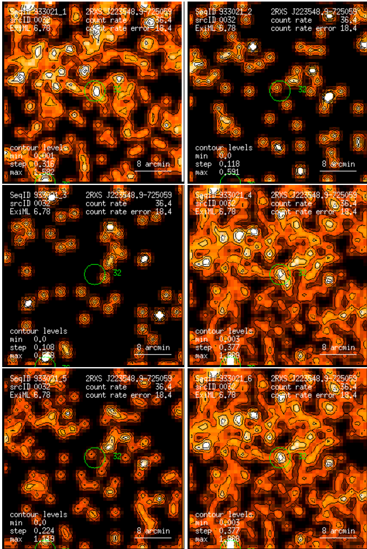
Figure 32: RASS 933021: detection 0032: band rate images, Gaussian filter: (1) PSPC channels 11 – 41, (2) 52 – 90, (3) 91 – 201, (4) 11 – 235, (5) 52 – 201, (6) 11 – 201. Broad band rates in counts/ks. Band rate contour levels in counts/ks/arcmin 2 .
