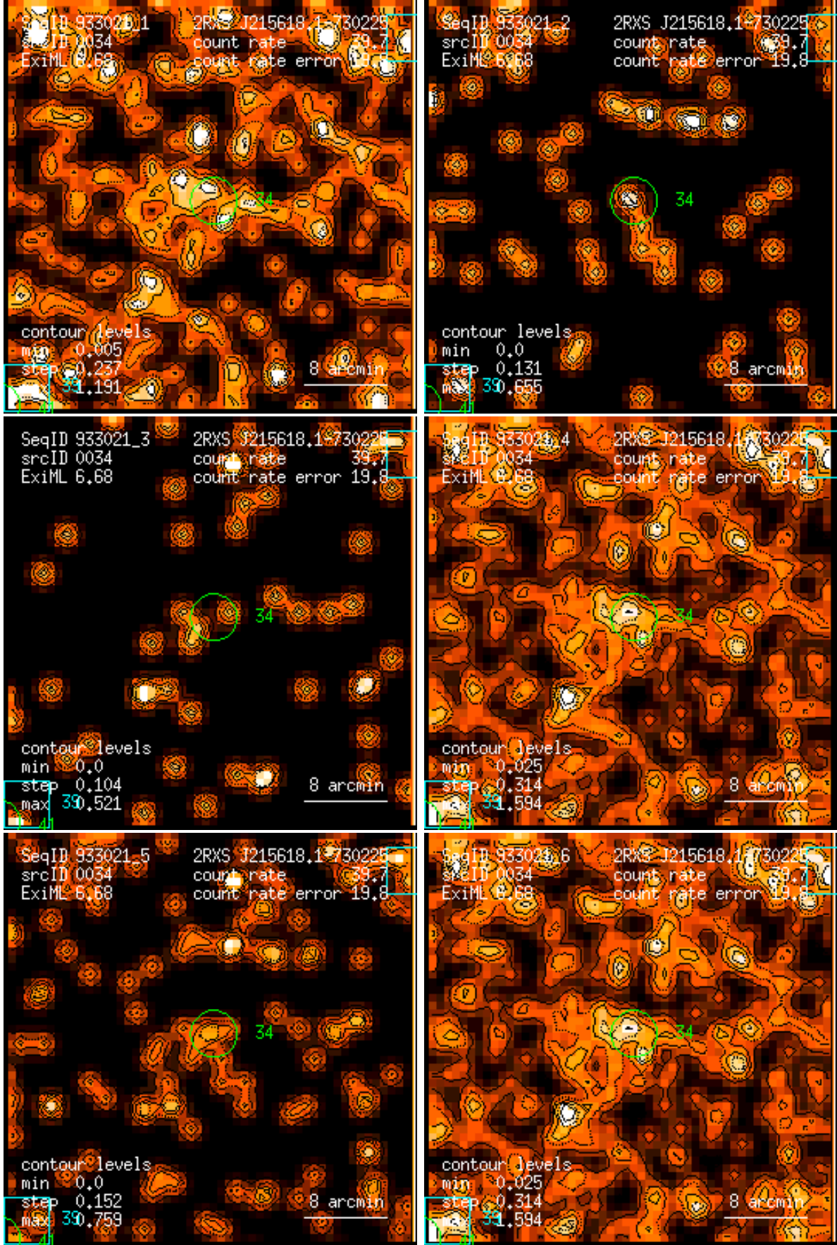
Figure 34: RASS 933021: detection 0034: band rate images, Gaussian filter: (1) PSPC channels 11 – 41, (2) 52 – 90, (3) 91 – 201, (4) 11 – 235, (5) 52 – 201, (6) 11 – 201. Broad band rates in counts/ks. Band rate contour levels in counts/ks/arcmin 2 .
