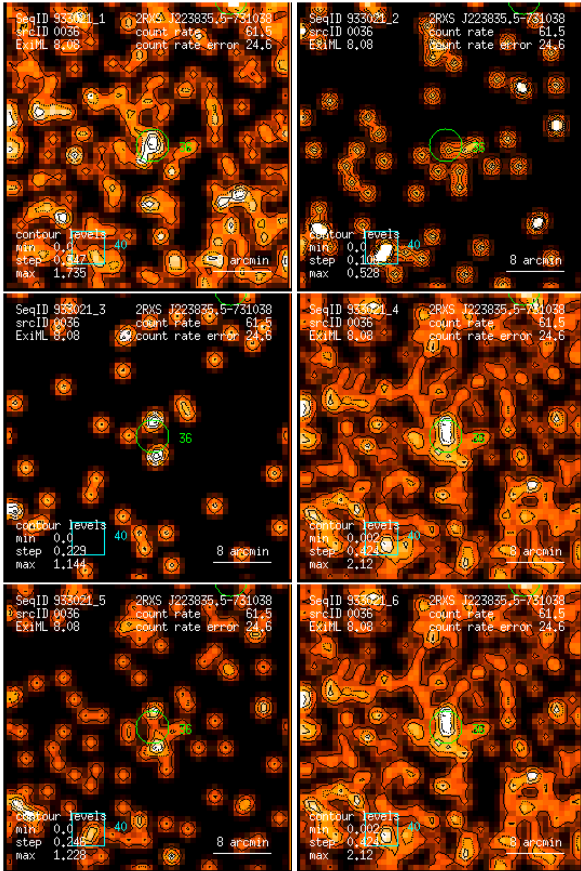
Figure 36: RASS 933021: detection 0036: band rate images, Gaussian filter: (1) PSPC channels 11 – 41, (2) 52 – 90, (3) 91 – 201, (4) 11 – 235, (5) 52 – 201, (6) 11 – 201. Broad band rates in counts/ks. Band rate contour levels in counts/ks/arcmin 2 .
