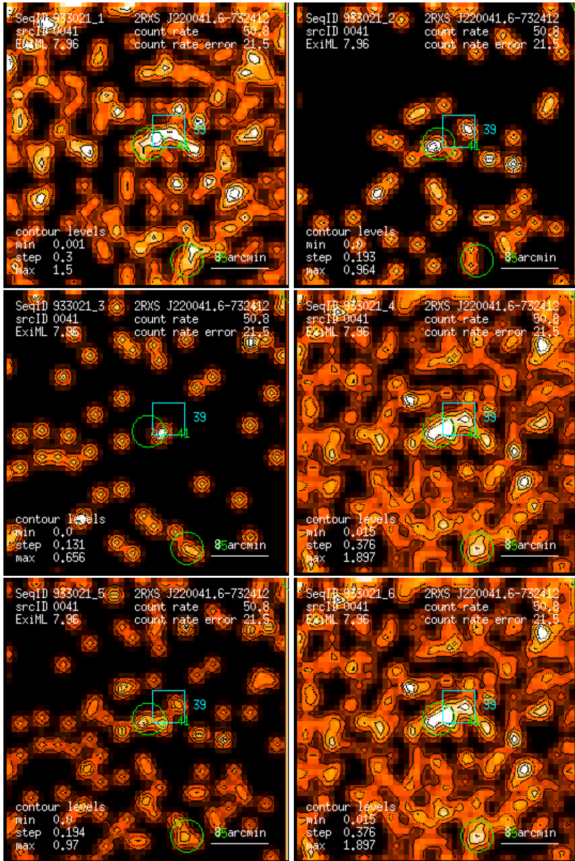
Figure 41: RASS 933021: detection 0041: band rate images, Gaussian filter: (1) PSPC channels 11 – 41, (2) 52 – 90, (3) 91 – 201, (4) 11 – 235, (5) 52 – 201, (6) 11 – 201. Broad band rates in counts/ks. Band rate contour levels in counts/ks/arcmin 2 .
