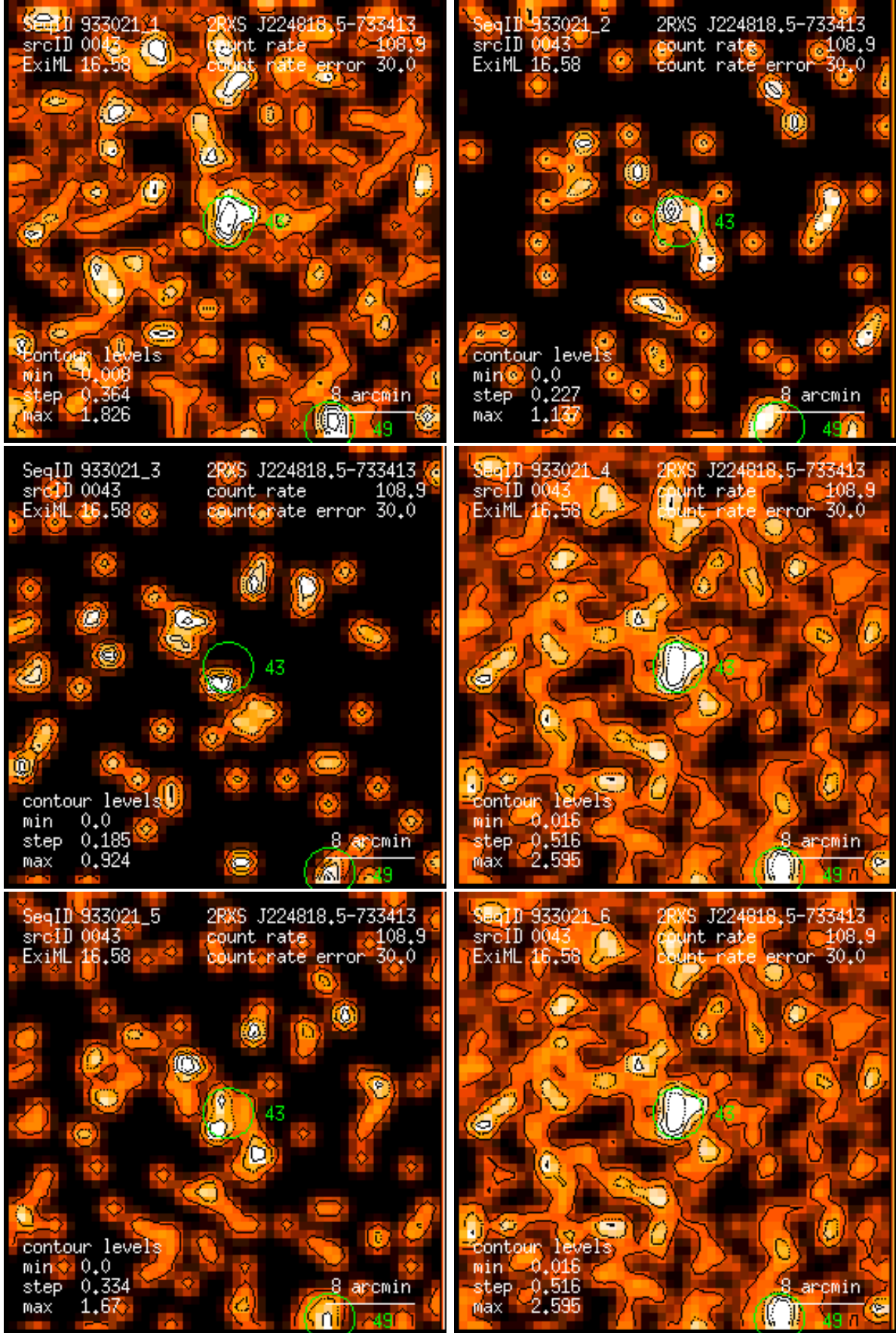
Figure 43: RASS 933021: detection 0043: band rate images, Gaussian filter: (1) PSPC channels 11 – 41, (2) 52 – 90, (3) 91 – 201, (4) 11 – 235, (5) 52 – 201, (6) 11 – 201. Broad band rates in counts/ks. Band rate contour levels in counts/ks/arcmin 2 .
