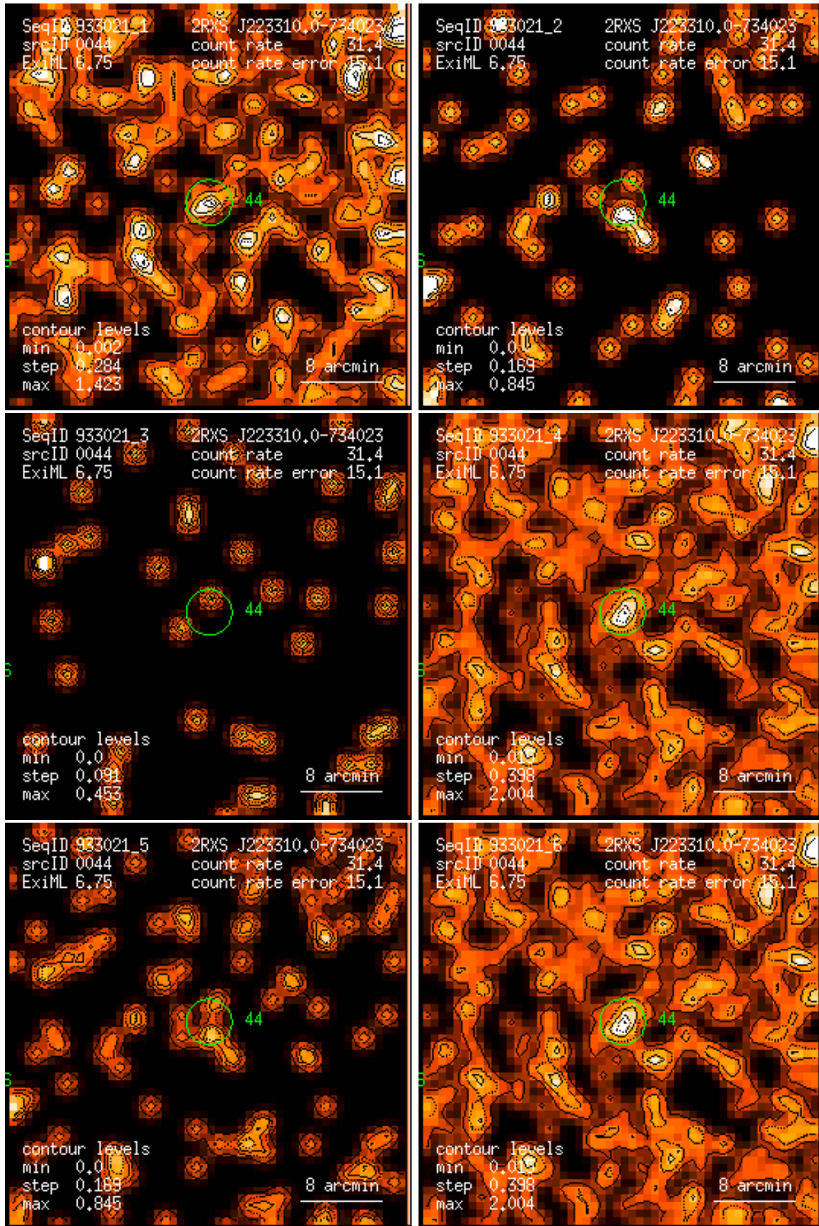
Figure 44: RASS 933021: detection 0044: band rate images, Gaussian filter: (1) PSPC channels 11 – 41, (2) 52 – 90, (3) 91 – 201, (4) 11 – 235, (5) 52 – 201, (6) 11 – 201. Broad band rates in counts/ks. Band rate contour levels in counts/ks/arcmin 2 .
