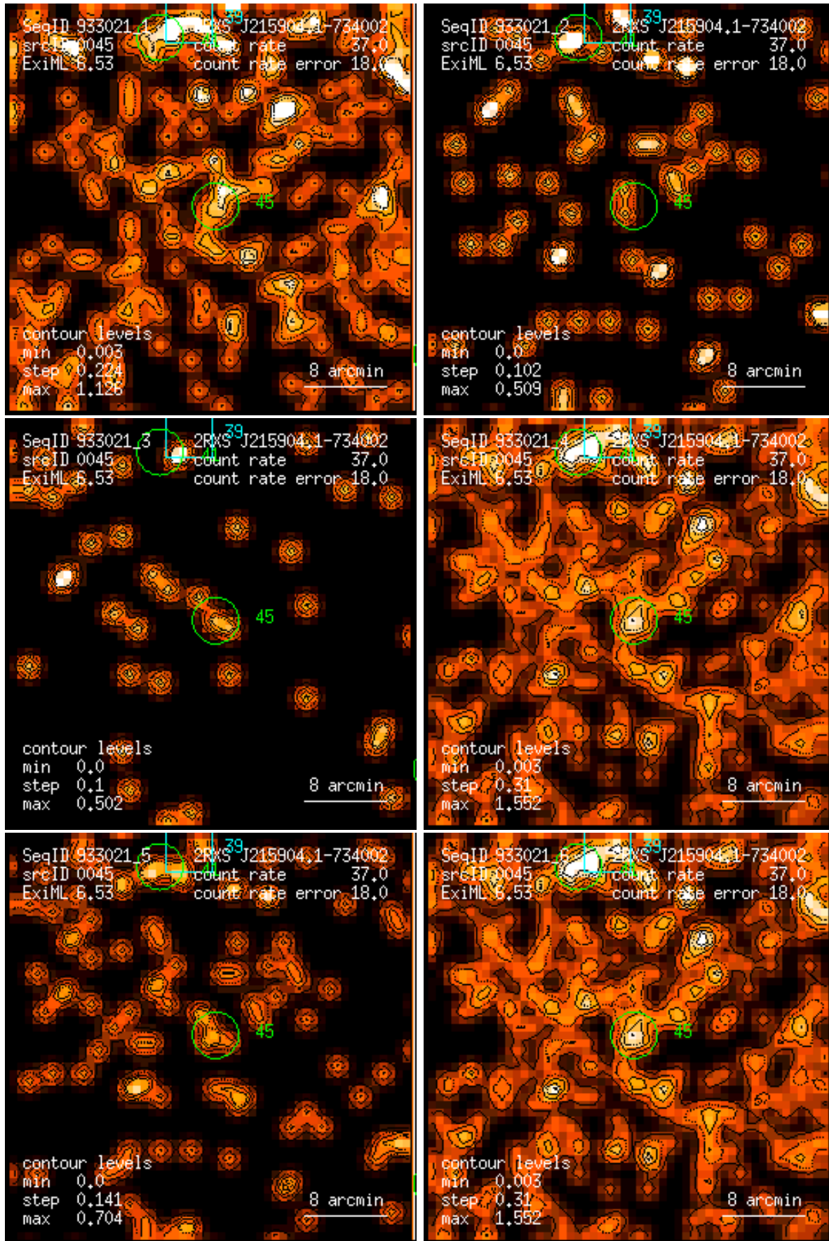
Figure 45: RASS 933021: detection 0045: band rate images, Gaussian filter: (1) PSPC channels 11 – 41, (2) 52 – 90, (3) 91 – 201, (4) 11 – 235, (5) 52 – 201, (6) 11 – 201. Broad band rates in counts/ks. Band rate contour levels in counts/ks/arcmin 2 .
