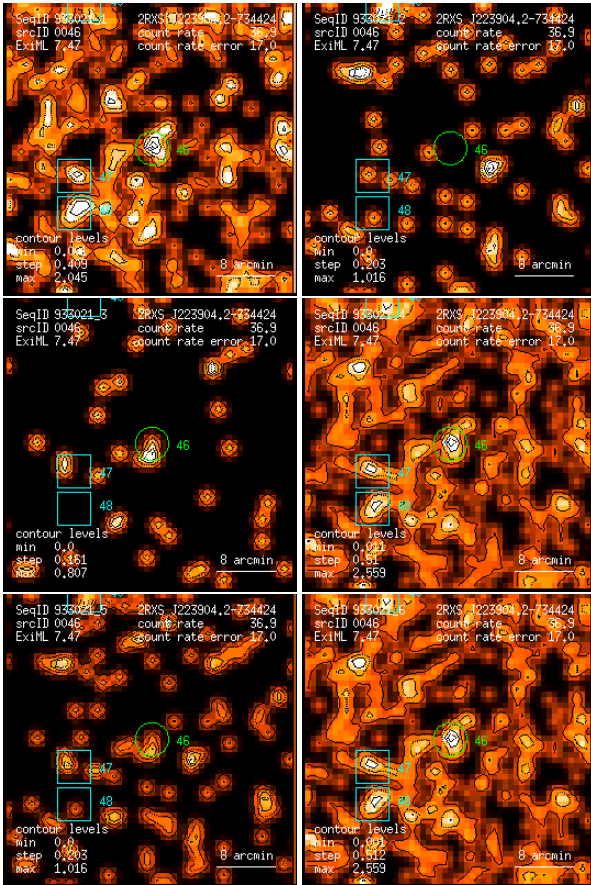
Figure 46: RASS 933021: detection 0046: band rate images, Gaussian filter: (1) PSPC channels 11 – 41, (2) 52 – 90, (3) 91 – 201, (4) 11 – 235, (5) 52 – 201, (6) 11 – 201. Broad band rates in counts/ks. Band rate contour levels in counts/ks/arcmin 2 .
