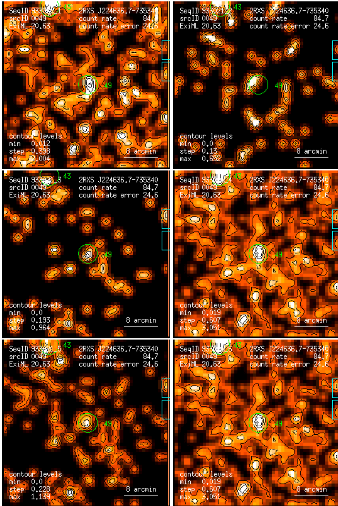
Figure 49: RASS 933021: detection 0049: band rate images, Gaussian filter: (1) PSPC channels 11 – 41, (2) 52 – 90, (3) 91 – 201, (4) 11 – 235, (5) 52 – 201, (6) 11 – 201. Broad band rates in counts/ks. Band rate contour levels in counts/ks/arcmin 2 .
