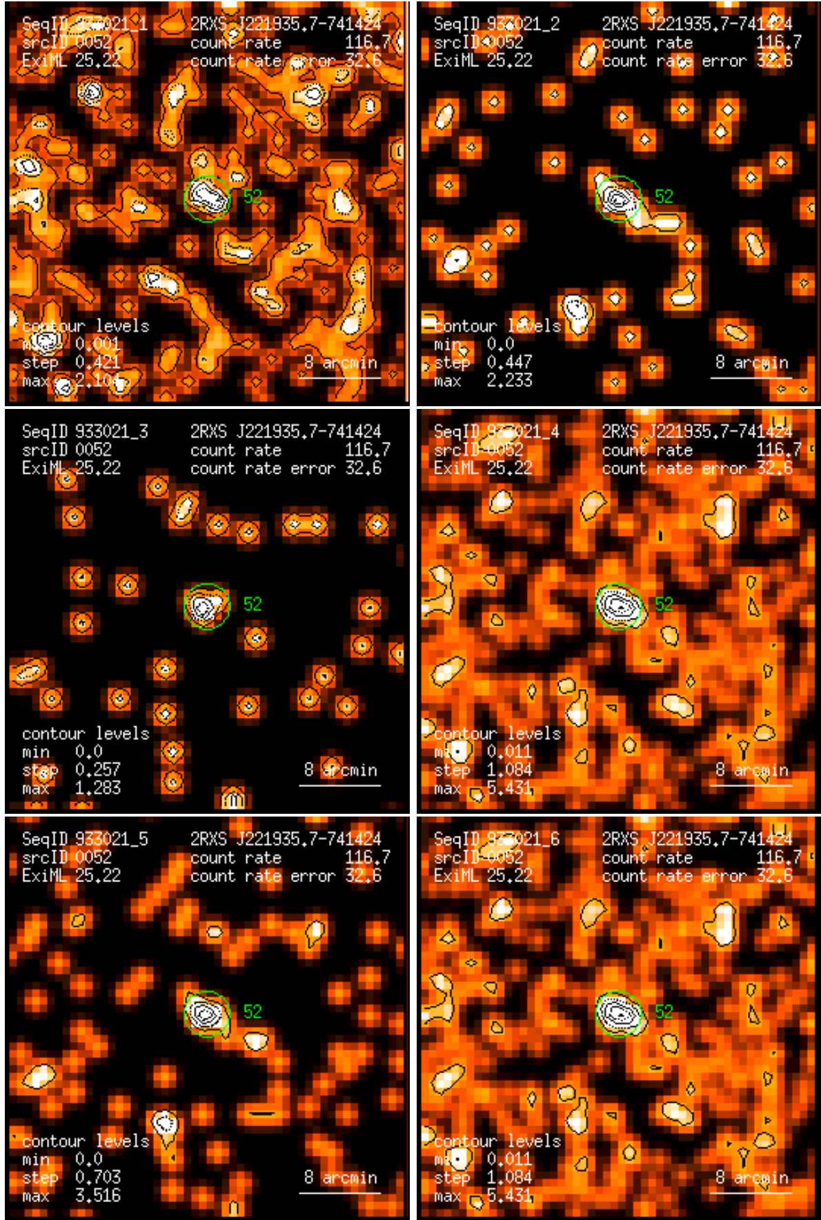
Figure 52: RASS 933021: detection 0052: band rate images, Gaussian filter: (1) PSPC channels 11 – 41, (2) 52 – 90, (3) 91 – 201, (4) 11 – 235, (5) 52 – 201, (6) 11 – 201. Broad band rates in counts/ks. Band rate contour levels in counts/ks/arcmin 2 .
