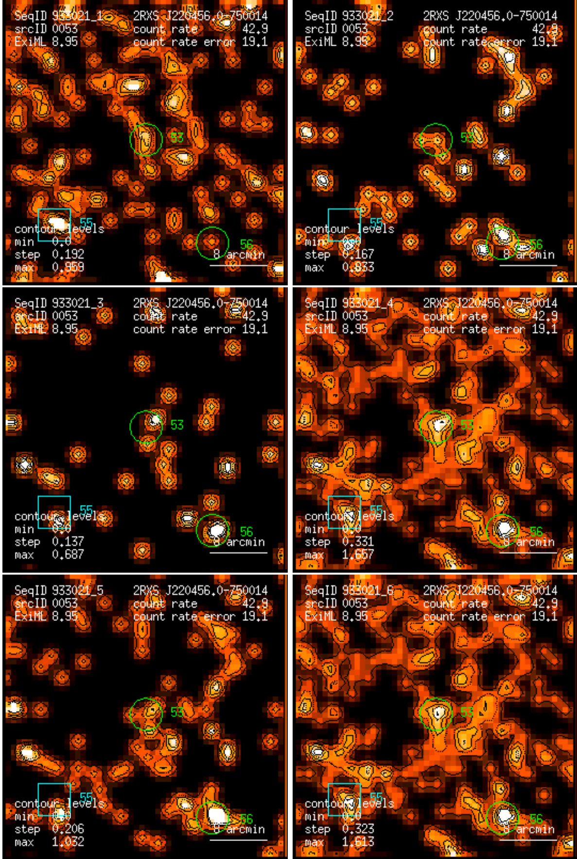
Figure 53: RASS 933021: detection 0053: band rate images, Gaussian filter: (1) PSPC channels 11 – 41, (2) 52 – 90, (3) 91 – 201, (4) 11 – 235, (5) 52 – 201, (6) 11 – 201. Broad band rates in counts/ks. Band rate contour levels in counts/ks/arcmin 2 .
