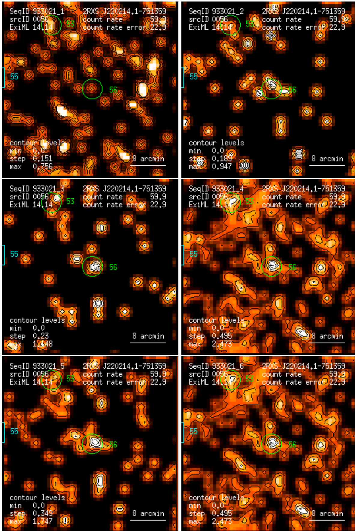
Figure 56: RASS 933021: detection 0056: band rate images, Gaussian filter: (1) PSPC channels 11 – 41, (2) 52 – 90, (3) 91 – 201, (4) 11 – 235, (5) 52 – 201, (6) 11 – 201. Broad band rates in counts/ks. Band rate contour levels in counts/ks/arcmin 2 .
