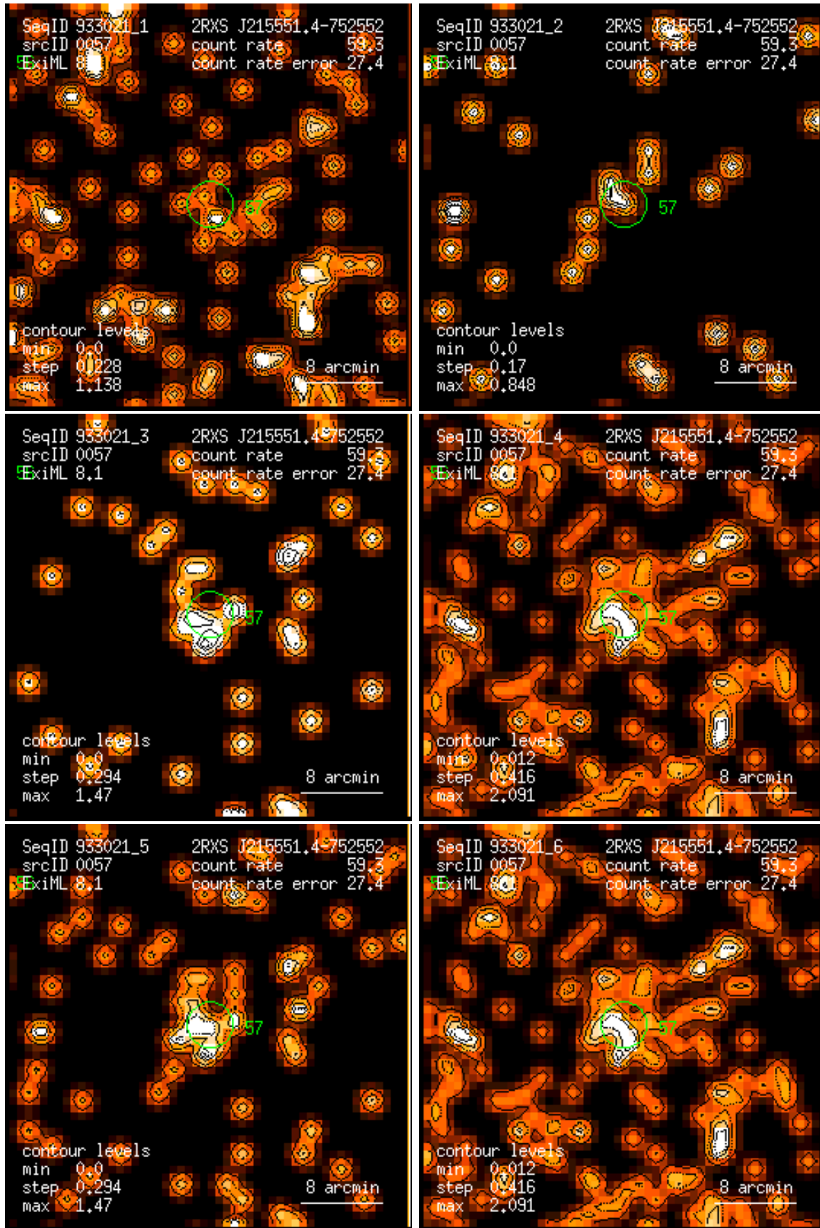
Figure 57: RASS 933021: detection 0057: band rate images, Gaussian filter: (1) PSPC channels 11 – 41, (2) 52 – 90, (3) 91 – 201, (4) 11 – 235, (5) 52 – 201, (6) 11 – 201. Broad band rates in counts/ks. Band rate contour levels in counts/ks/arcmin 2 .
