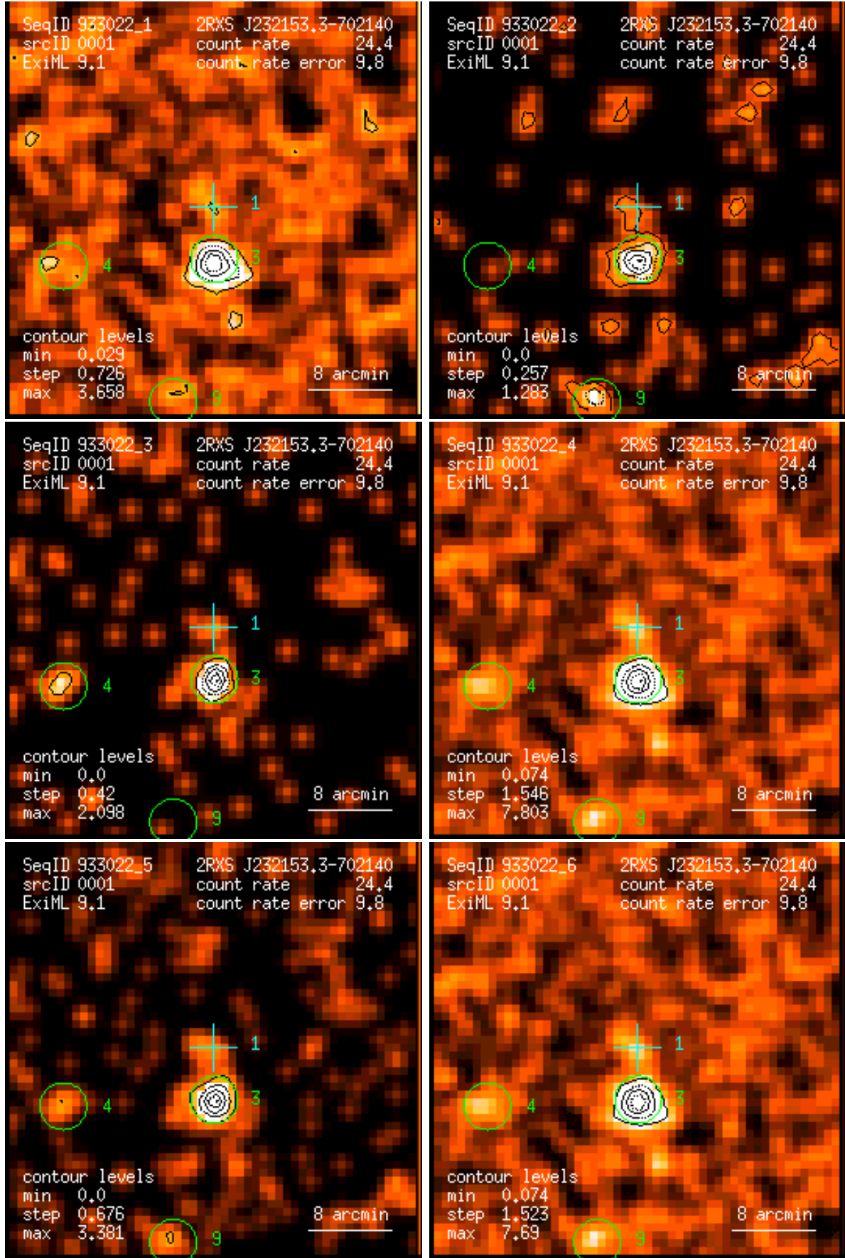
Figure 1: RASS 933022: detection 0001: band rate images, Gaussian filter: (1) PSPC channels 11 – 41, (2) 52 – 90, (3) 91 – 201, (4) 11 – 235, (5) 52 – 201, (6) 11 – 201. Broad band rates in counts/ks. Band rate contour levels in counts/ks/arcmin 2 .
