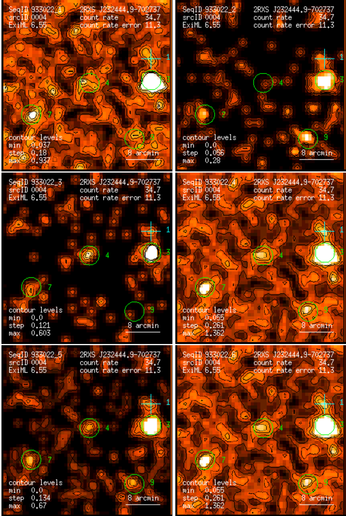
Figure 4: RASS 933022: detection 0004: band rate images, Gaussian filter: (1) PSPC channels 11 – 41, (2) 52 – 90, (3) 91 – 201, (4) 11 – 235, (5) 52 – 201, (6) 11 – 201. Broad band rates in counts/ks. Band rate contour levels in counts/ks/arcmin 2 .
