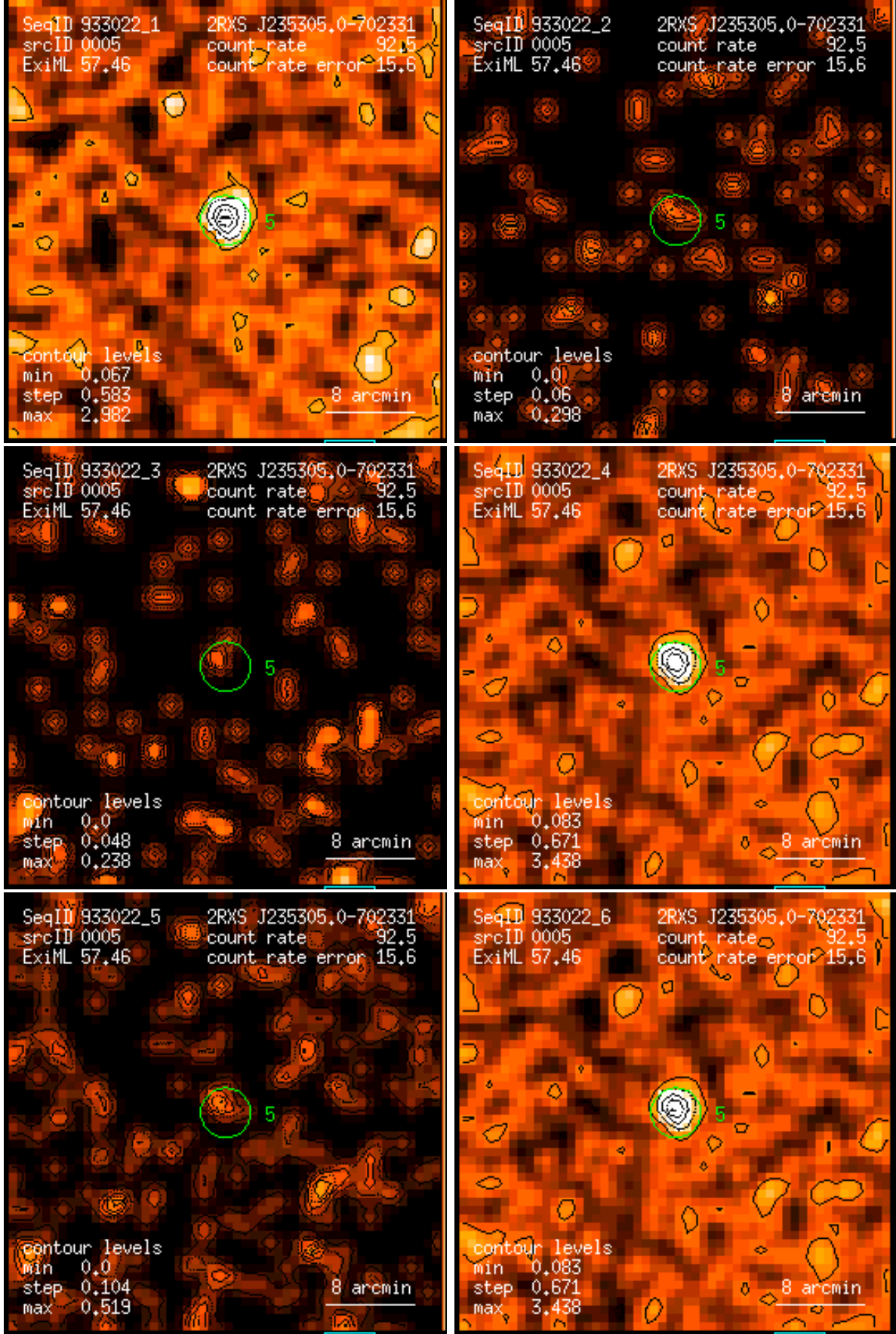
Figure 5: RASS 933022: detection 0005: band rate images, Gaussian filter: (1) PSPC channels 11 – 41, (2) 52 – 90, (3) 91 – 201, (4) 11 – 235, (5) 52 – 201, (6) 11 – 201. Broad band rates in counts/ks. Band rate contour levels in counts/ks/arcmin 2 .
