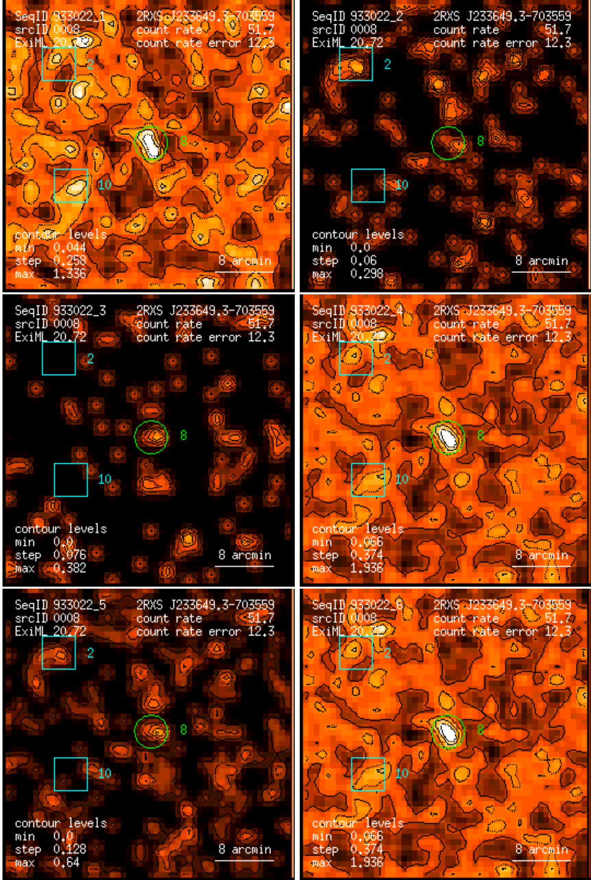
Figure 8: RASS 933022: detection 0008: band rate images, Gaussian filter: (1) PSPC channels 11 – 41, (2) 52 – 90, (3) 91 – 201, (4) 11 – 235, (5) 52 – 201, (6) 11 – 201. Broad band rates in counts/ks. Band rate contour levels in counts/ks/arcmin 2 .
