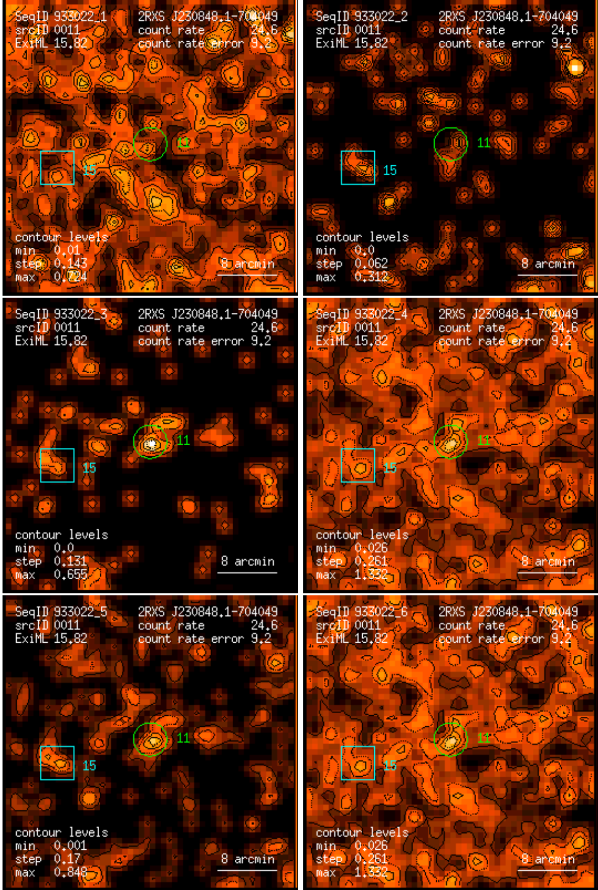
Figure 11: RASS 933022: detection 0011: band rate images, Gaussian filter: (1) PSPC channels 11 – 41, (2) 52 – 90, (3) 91 – 201, (4) 11 – 235, (5) 52 – 201, (6) 11 – 201. Broad band rates in counts/ks. Band rate contour levels in counts/ks/arcmin 2 .
