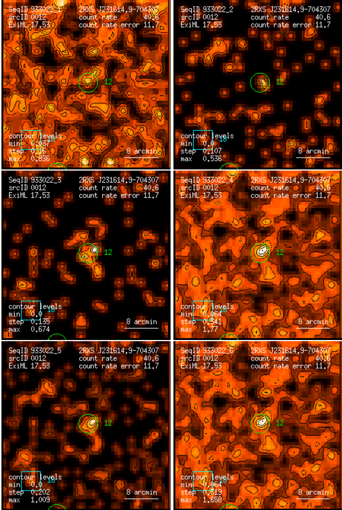
Figure 12: RASS 933022: detection 0012: band rate images, Gaussian filter: (1) PSPC channels 11 – 41, (2) 52 – 90, (3) 91 – 201, (4) 11 – 235, (5) 52 – 201, (6) 11 – 201. Broad band rates in counts/ks. Band rate contour levels in counts/ks/arcmin 2 .
