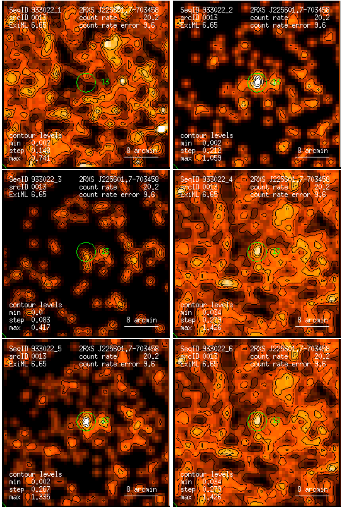
Figure 13: RASS 933022: detection 0013: band rate images, Gaussian filter: (1) PSPC channels 11 – 41, (2) 52 – 90, (3) 91 – 201, (4) 11 – 235, (5) 52 – 201, (6) 11 – 201. Broad band rates in counts/ks. Band rate contour levels in counts/ks/arcmin 2 .
