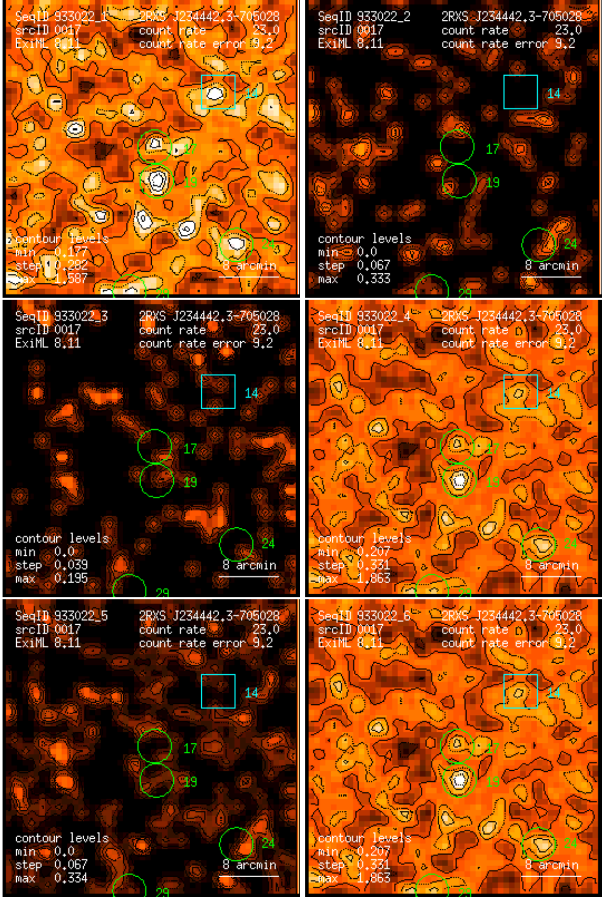
Figure 17: RASS 933022: detection 0017: band rate images, Gaussian filter: (1) PSPC channels 11 – 41, (2) 52 – 90, (3) 91 – 201, (4) 11 – 235, (5) 52 – 201, (6) 11 – 201. Broad band rates in counts/ks. Band rate contour levels in counts/ks/arcmin 2 .
