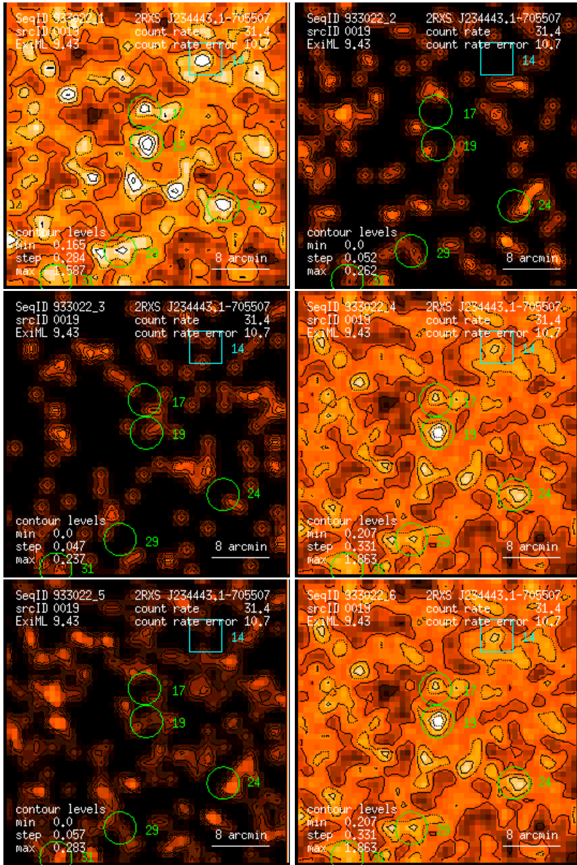
Figure 19: RASS 933022: detection 0019: band rate images, Gaussian filter: (1) PSPC channels 11 – 41, (2) 52 – 90, (3) 91 – 201, (4) 11 – 235, (5) 52 – 201, (6) 11 – 201. Broad band rates in counts/ks. Band rate contour levels in counts/ks/arcmin 2 .
