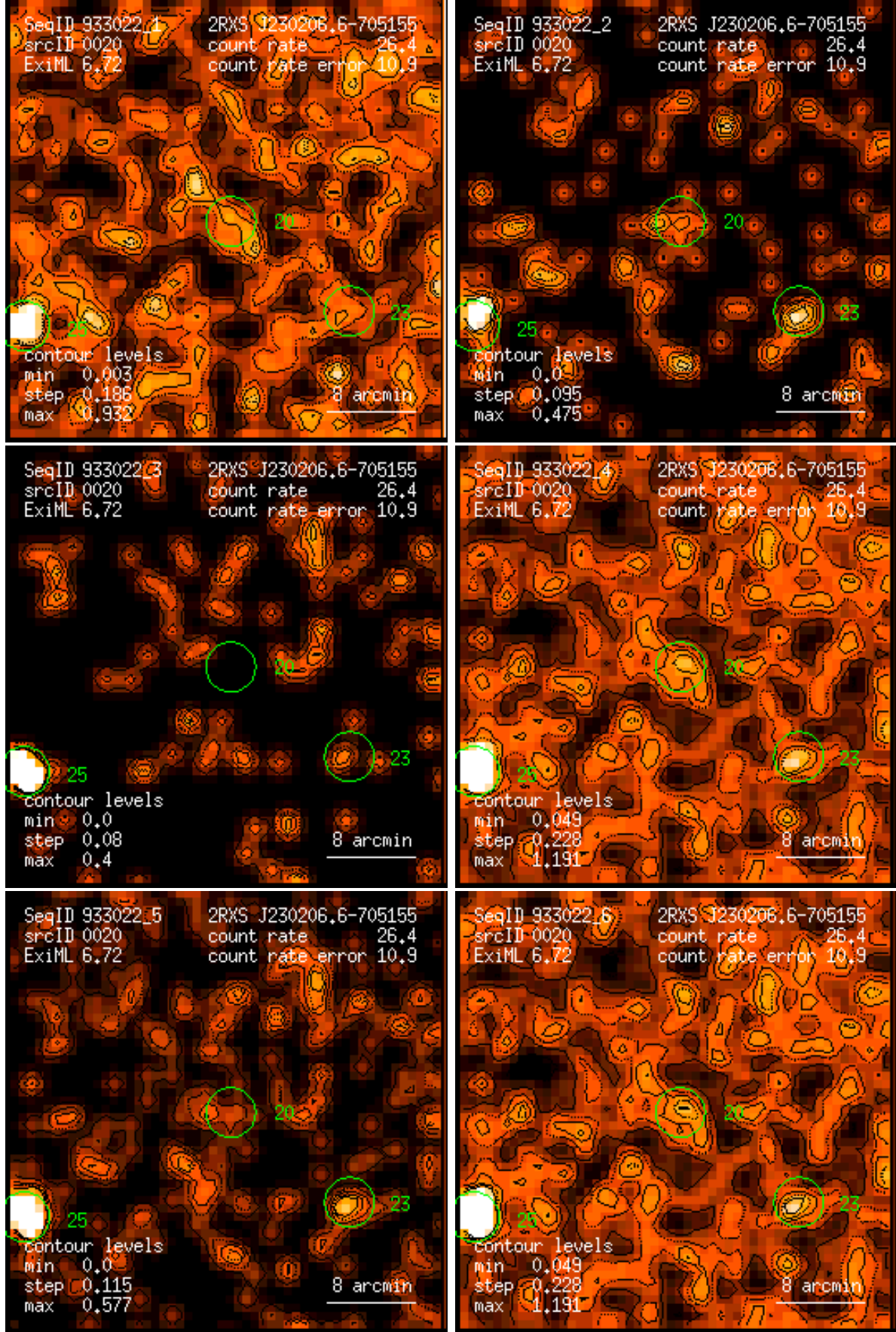
Figure 20: RASS 933022: detection 0020: band rate images, Gaussian filter: (1) PSPC channels 11 – 41, (2) 52 – 90, (3) 91 – 201, (4) 11 – 235, (5) 52 – 201, (6) 11 – 201. Broad band rates in counts/ks. Band rate contour levels in counts/ks/arcmin 2 .
