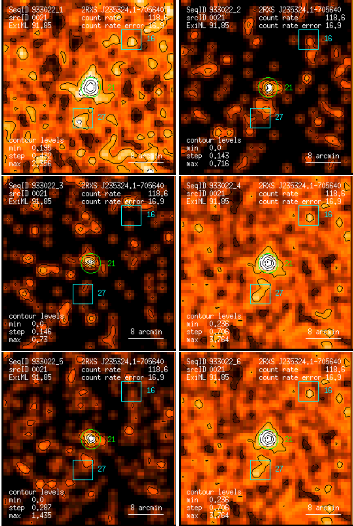
Figure 21: RASS 933022: detection 0021: band rate images, Gaussian filter: (1) PSPC channels 11 – 41, (2) 52 – 90, (3) 91 – 201, (4) 11 – 235, (5) 52 – 201, (6) 11 – 201. Broad band rates in counts/ks. Band rate contour levels in counts/ks/arcmin 2 .
