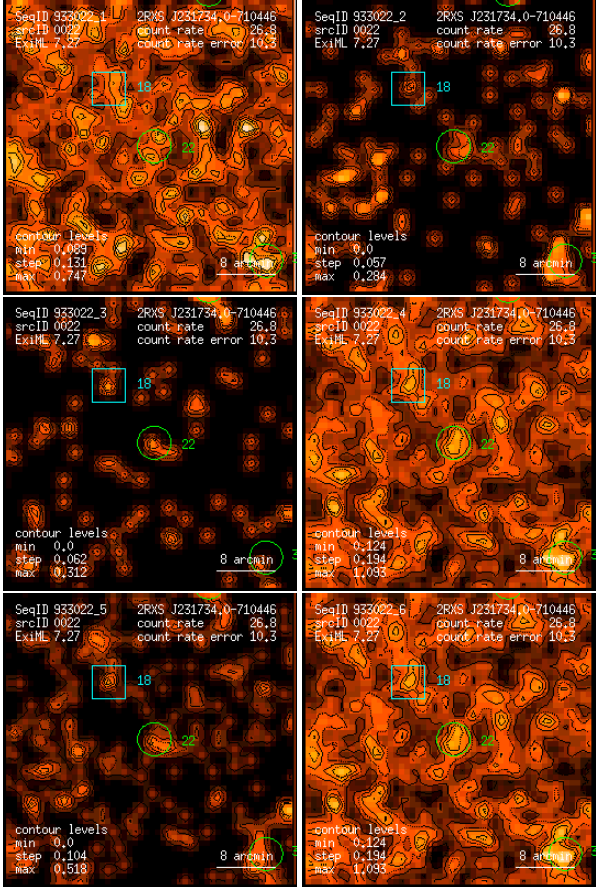
Figure 22: RASS 933022: detection 0022: band rate images, Gaussian filter: (1) PSPC channels 11 – 41, (2) 52 – 90, (3) 91 – 201, (4) 11 – 235, (5) 52 – 201, (6) 11 – 201. Broad band rates in counts/ks. Band rate contour levels in counts/ks/arcmin 2 .
