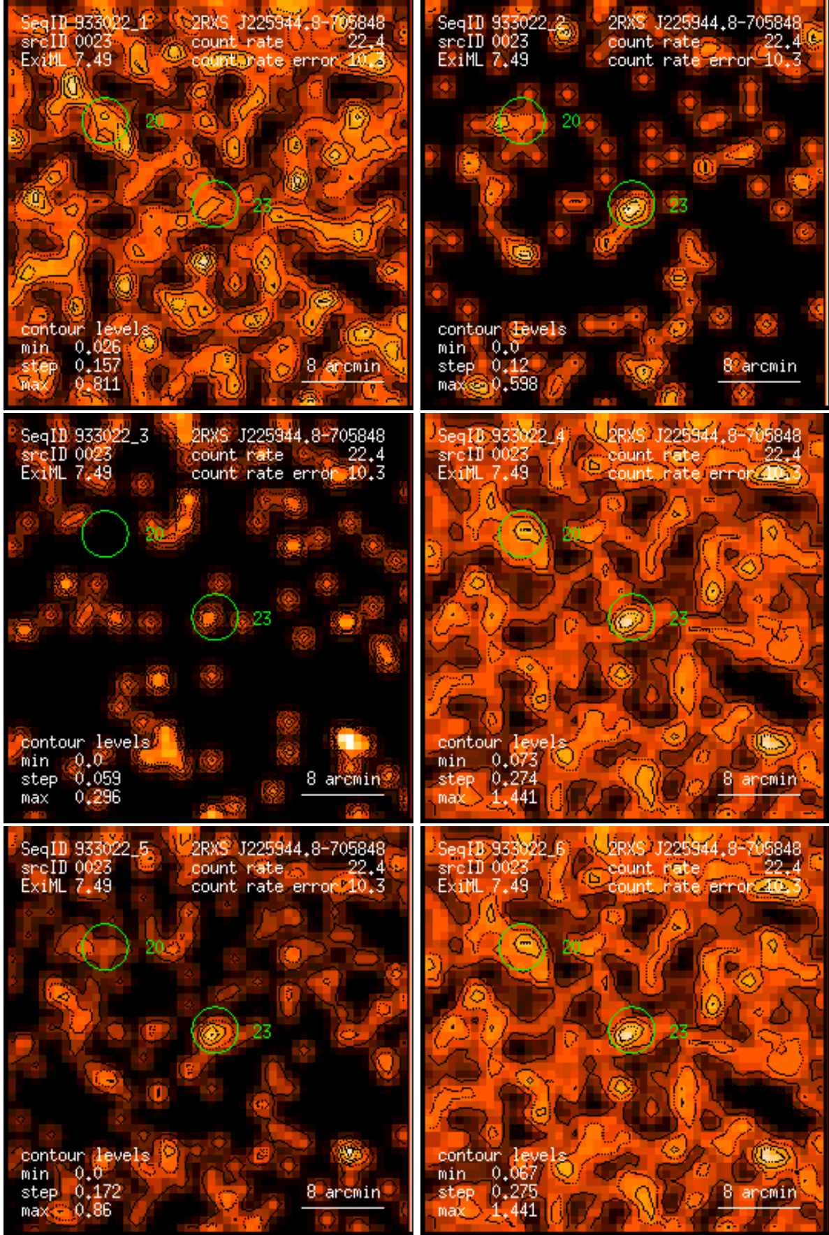
Figure 23: RASS 933022: detection 0023: band rate images, Gaussian filter: (1) PSPC channels 11 – 41, (2) 52 – 90, (3) 91 – 201, (4) 11 – 235, (5) 52 – 201, (6) 11 – 201. Broad band rates in counts/ks. Band rate contour levels in counts/ks/arcmin 2 .
