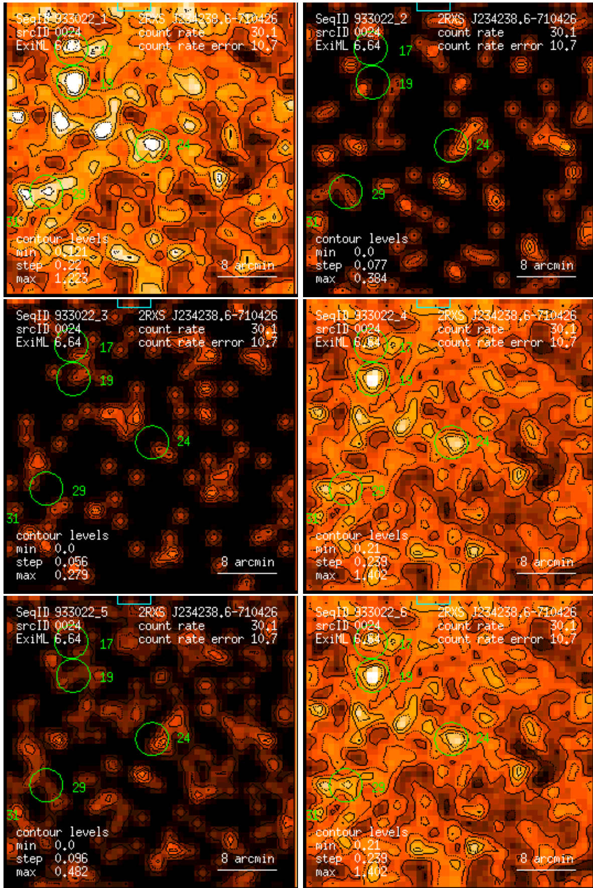
Figure 24: RASS 933022: detection 0024: band rate images, Gaussian filter: (1) PSPC channels 11 – 41, (2) 52 – 90, (3) 91 – 201, (4) 11 – 235, (5) 52 – 201, (6) 11 – 201. Broad band rates in counts/ks. Band rate contour levels in counts/ks/arcmin 2 .
