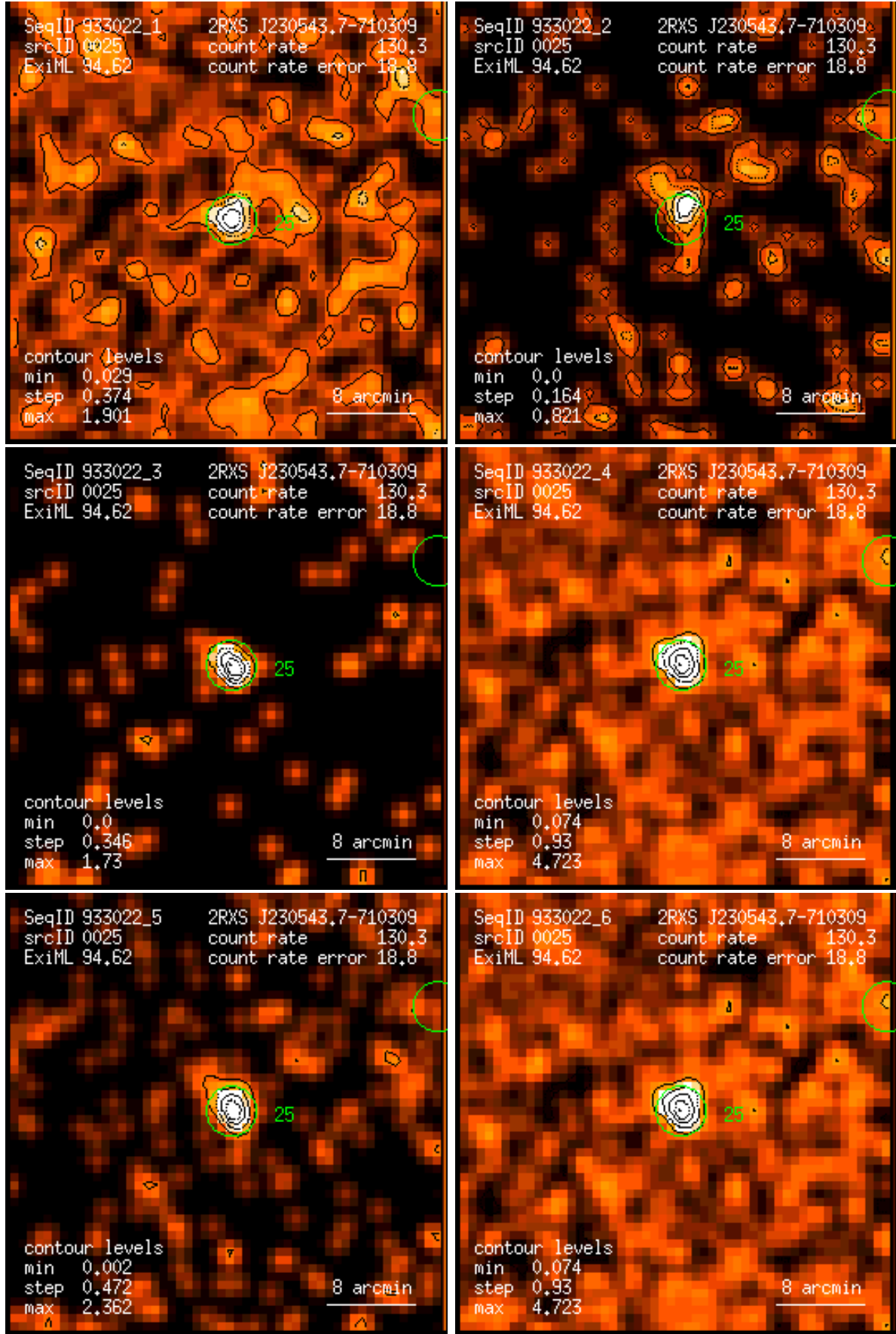
Figure 25: RASS 933022: detection 0025: band rate images, Gaussian filter: (1) PSPC channels 11 – 41, (2) 52 – 90, (3) 91 – 201, (4) 11 – 235, (5) 52 – 201, (6) 11 – 201. Broad band rates in counts/ks. Band rate contour levels in counts/ks/arcmin 2 .
