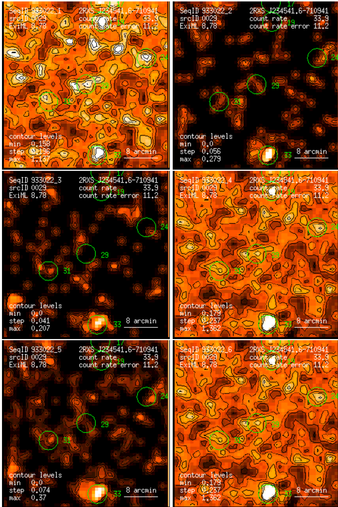
Figure 29: RASS 933022: detection 0029: band rate images, Gaussian filter: (1) PSPC channels 11 – 41, (2) 52 – 90, (3) 91 – 201, (4) 11 – 235, (5) 52 – 201, (6) 11 – 201. Broad band rates in counts/ks. Band rate contour levels in counts/ks/arcmin 2 .
