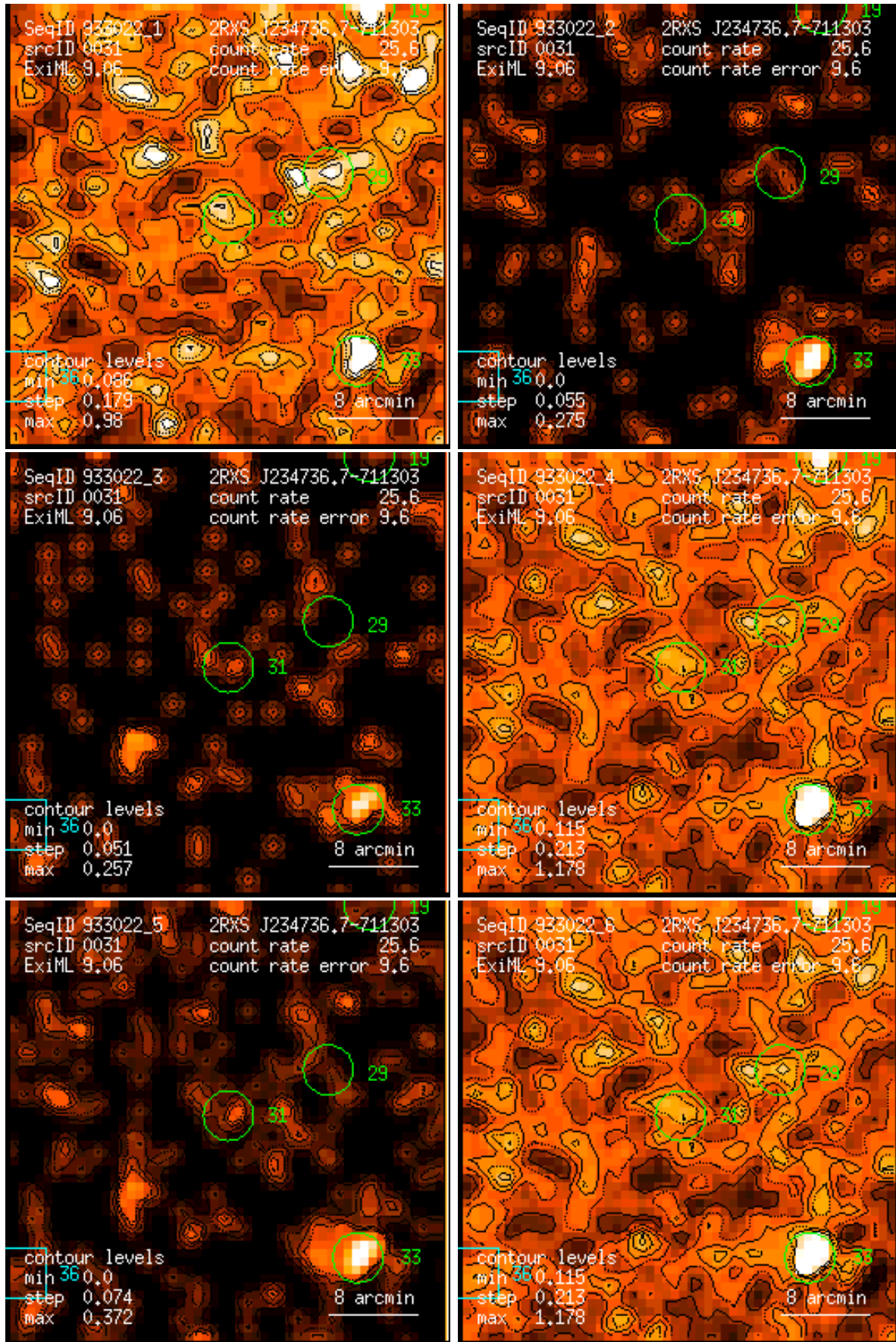
Figure 31: RASS 933022: detection 0031: band rate images, Gaussian filter: (1) PSPC channels 11 – 41, (2) 52 – 90, (3) 91 – 201, (4) 11 – 235, (5) 52 – 201, (6) 11 – 201. Broad band rates in counts/ks. Band rate contour levels in counts/ks/arcmin 2 .
