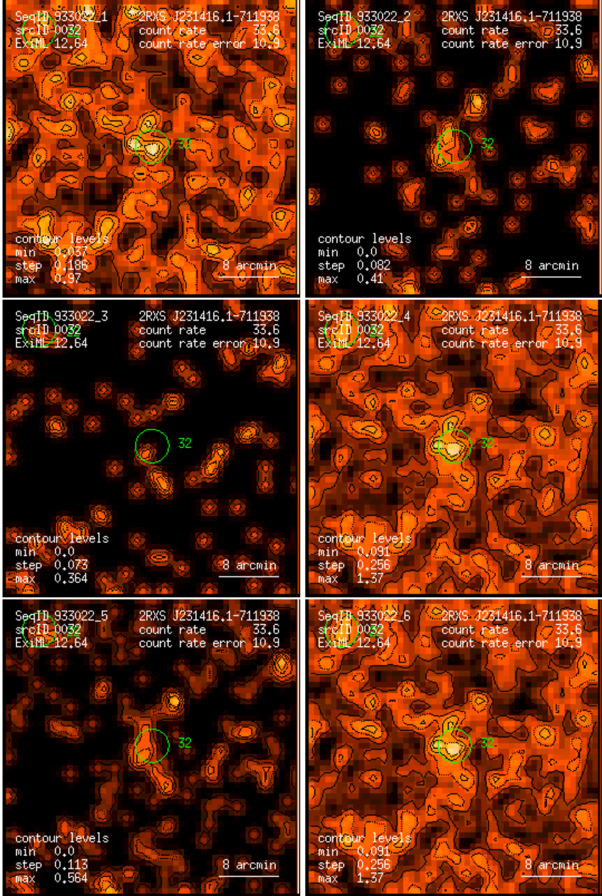
Figure 32: RASS 933022: detection 0032: band rate images, Gaussian filter: (1) PSPC channels 11 – 41, (2) 52 – 90, (3) 91 – 201, (4) 11 – 235, (5) 52 – 201, (6) 11 – 201. Broad band rates in counts/ks. Band rate contour levels in counts/ks/arcmin 2 .
