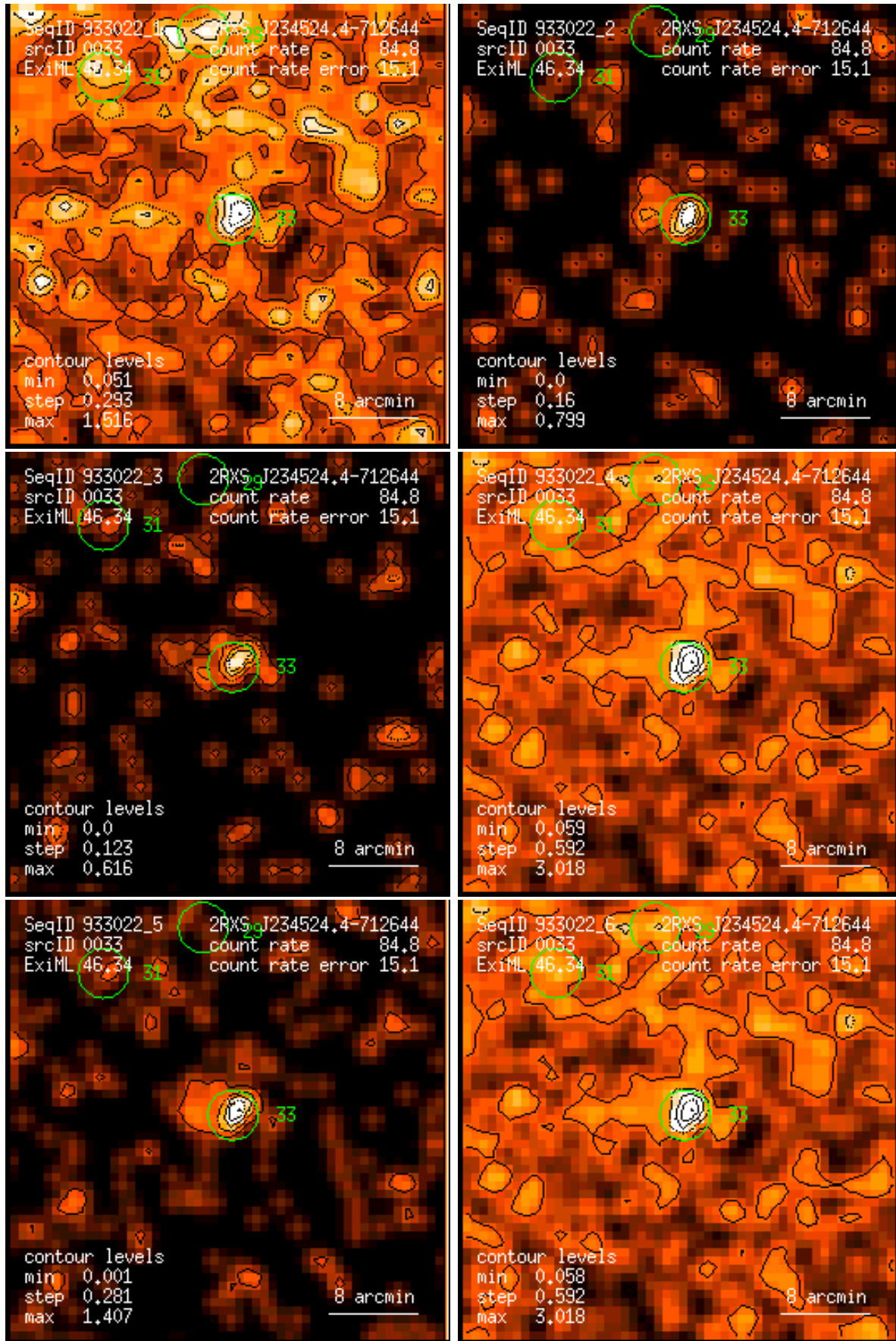
Figure 33: RASS 933022: detection 0033: band rate images, Gaussian filter: (1) PSPC channels 11 – 41, (2) 52 – 90, (3) 91 – 201, (4) 11 – 235, (5) 52 – 201, (6) 11 – 201. Broad band rates in counts/ks. Band rate contour levels in counts/ks/arcmin 2 .
