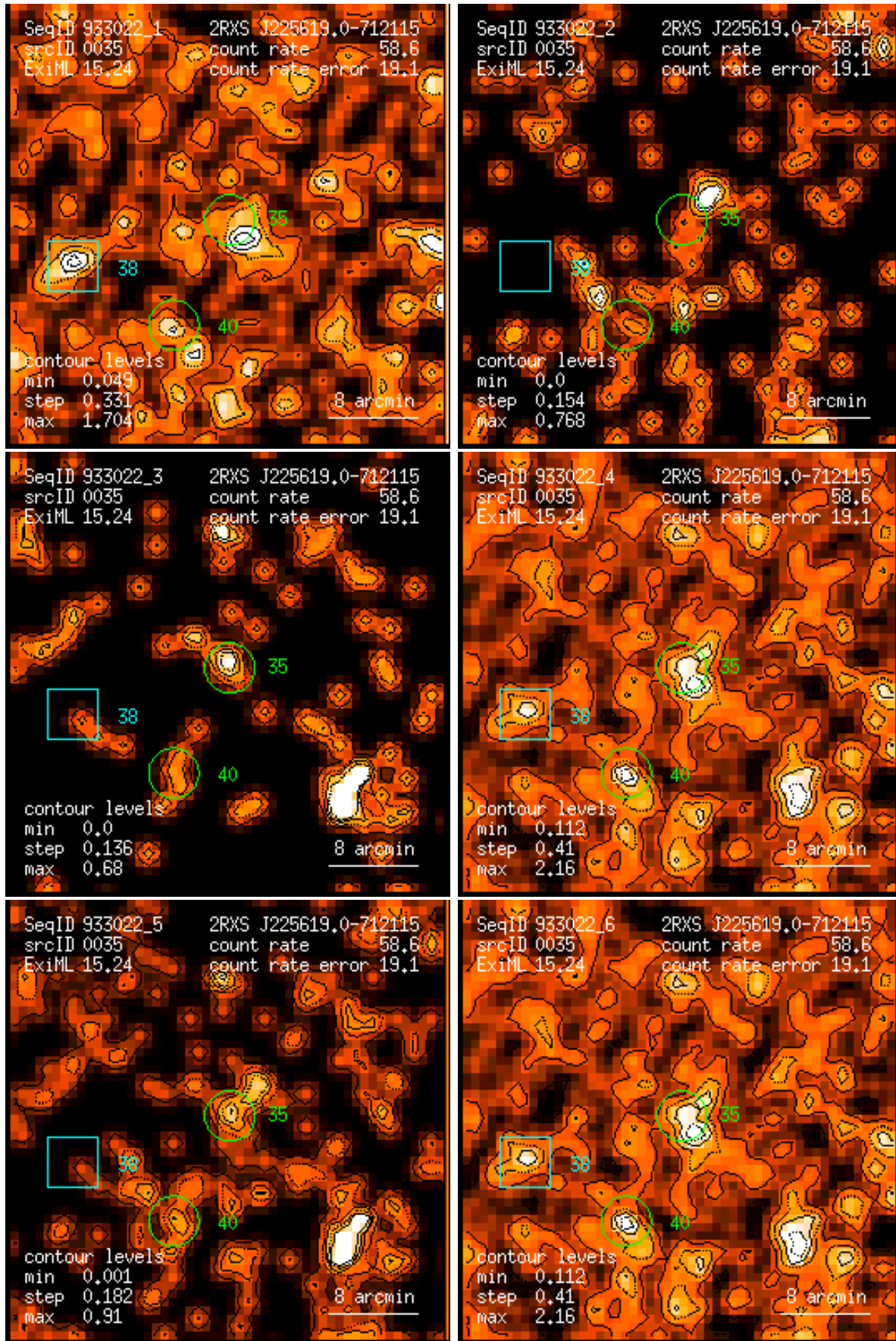
Figure 35: RASS 933022: detection 0035: band rate images, Gaussian filter: (1) PSPC channels 11 – 41, (2) 52 – 90, (3) 91 – 201, (4) 11 – 235, (5) 52 – 201, (6) 11 – 201. Broad band rates in counts/ks. Band rate contour levels in counts/ks/arcmin 2 .
