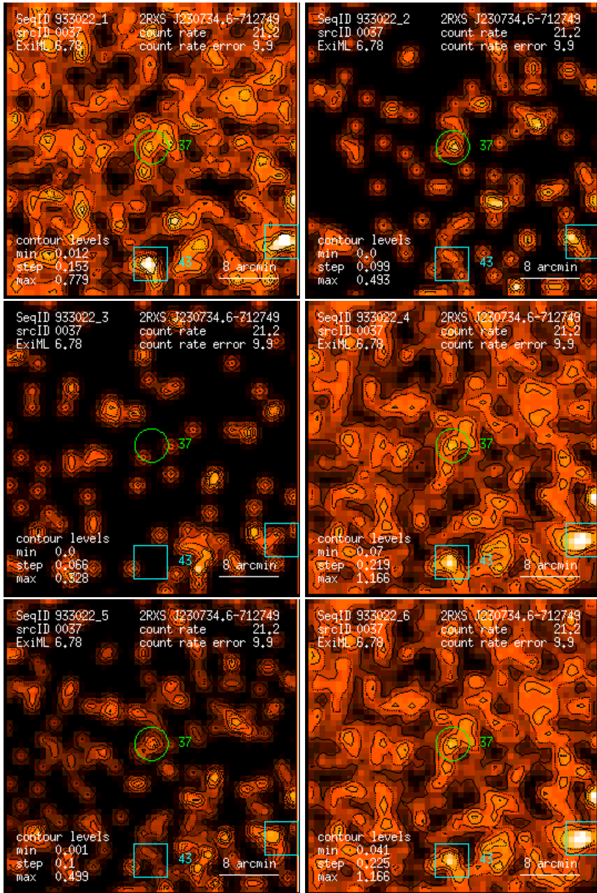
Figure 37: RASS 933022: detection 0037: band rate images, Gaussian filter: (1) PSPC channels 11 – 41, (2) 52 – 90, (3) 91 – 201, (4) 11 – 235, (5) 52 – 201, (6) 11 – 201. Broad band rates in counts/ks. Band rate contour levels in counts/ks/arcmin 2 .
