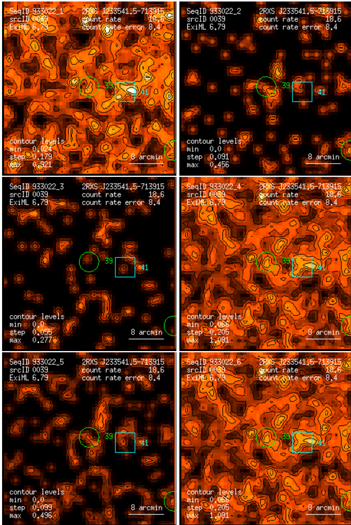
Figure 39: RASS 933022: detection 0039: band rate images, Gaussian filter: (1) PSPC channels 11 – 41, (2) 52 – 90, (3) 91 – 201, (4) 11 – 235, (5) 52 – 201, (6) 11 – 201. Broad band rates in counts/ks. Band rate contour levels in counts/ks/arcmin 2 .
