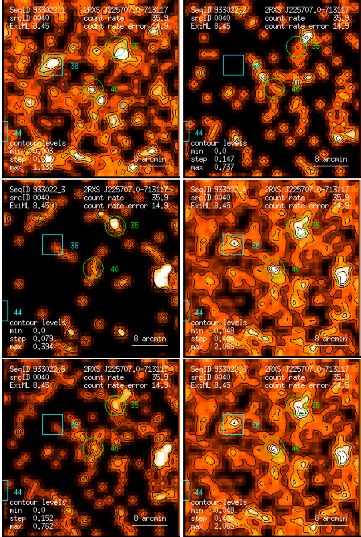
Figure 40: RASS 933022: detection 0040: band rate images, Gaussian filter: (1) PSPC channels 11 – 41, (2) 52 – 90, (3) 91 – 201, (4) 11 – 235, (5) 52 – 201, (6) 11 – 201. Broad band rates in counts/ks. Band rate contour levels in counts/ks/arcmin 2 .
