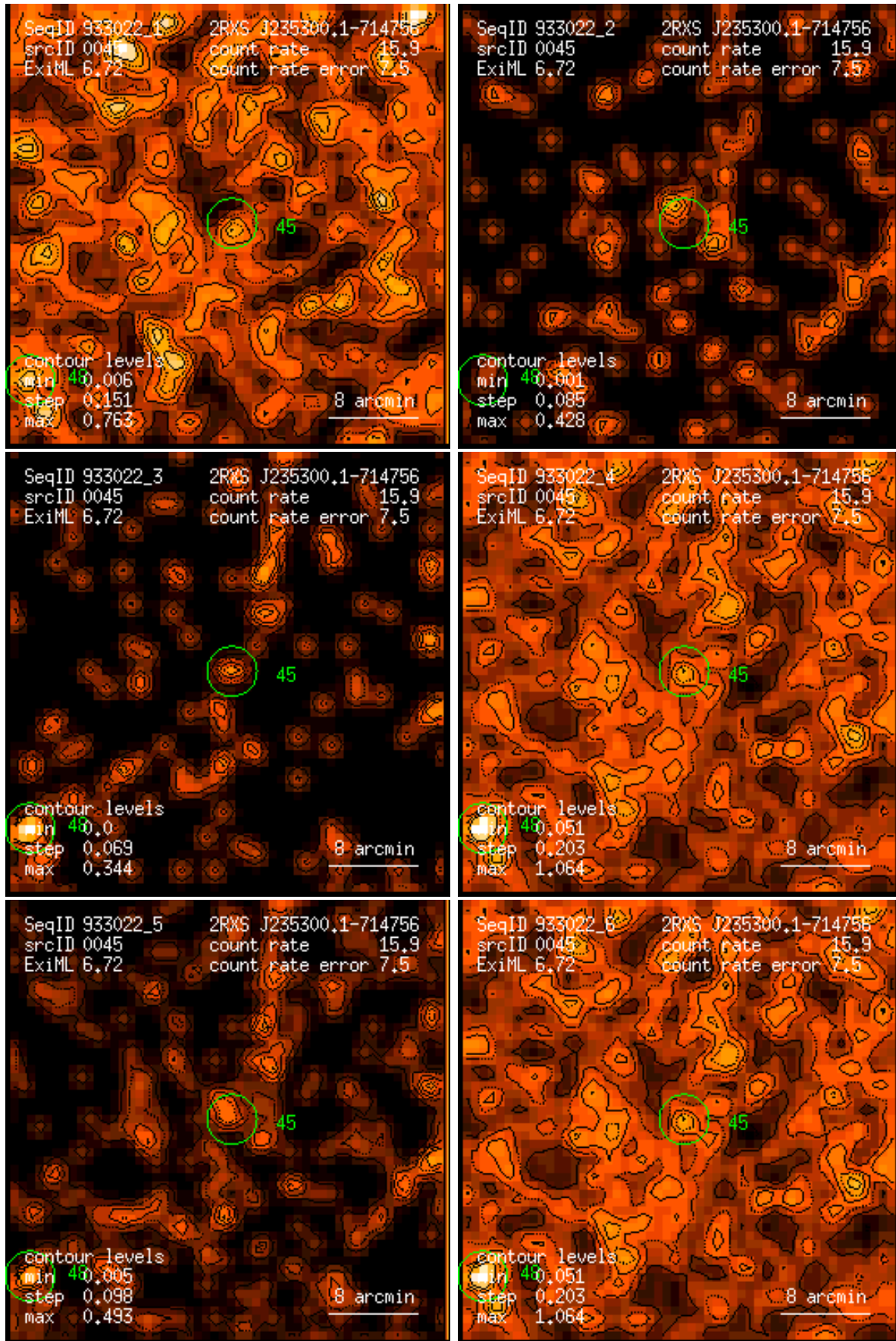
Figure 45: RASS 933022: detection 0045: band rate images, Gaussian filter: (1) PSPC channels 11 – 41, (2) 52 – 90, (3) 91 – 201, (4) 11 – 235, (5) 52 – 201, (6) 11 – 201. Broad band rates in counts/ks. Band rate contour levels in counts/ks/arcmin 2 .
