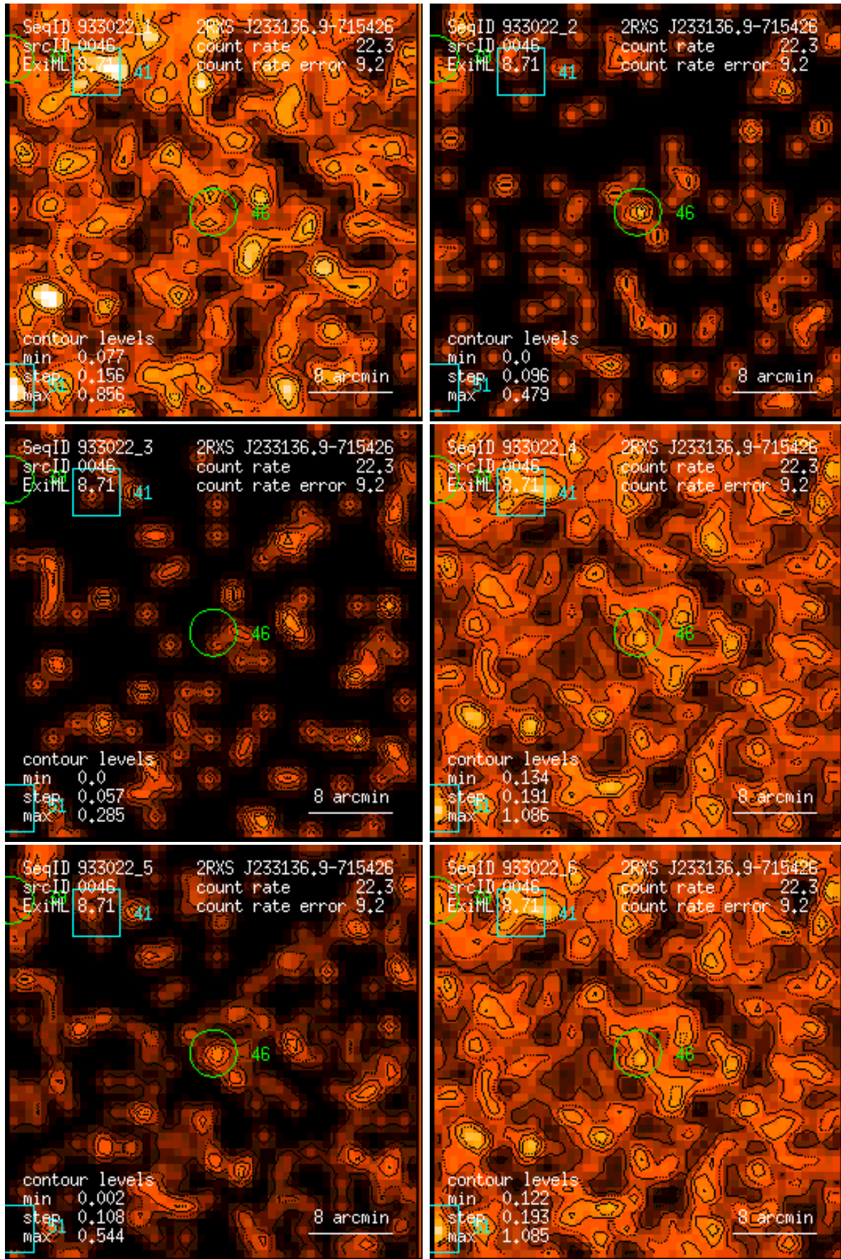
Figure 46: RASS 933022: detection 0046: band rate images, Gaussian filter: (1) PSPC channels 11 – 41, (2) 52 – 90, (3) 91 – 201, (4) 11 – 235, (5) 52 – 201, (6) 11 – 201. Broad band rates in counts/ks. Band rate contour levels in counts/ks/arcmin 2 .
