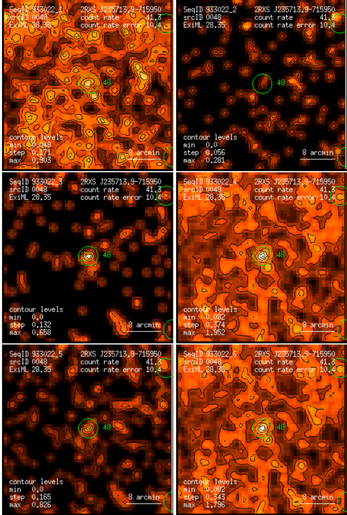
Figure 48: RASS 933022: detection 0048: band rate images, Gaussian filter: (1) PSPC channels 11 – 41, (2) 52 – 90, (3) 91 – 201, (4) 11 – 235, (5) 52 – 201, (6) 11 – 201. Broad band rates in counts/ks. Band rate contour levels in counts/ks/arcmin 2 .
