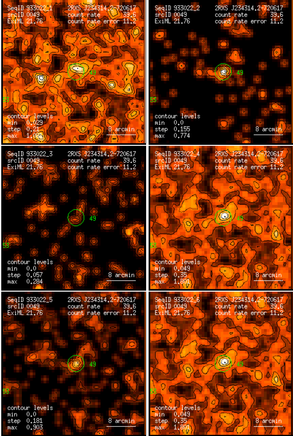
Figure 49: RASS 933022: detection 0049: band rate images, Gaussian filter: (1) PSPC channels 11 – 41, (2) 52 – 90, (3) 91 – 201, (4) 11 – 235, (5) 52 – 201, (6) 11 – 201. Broad band rates in counts/ks. Band rate contour levels in counts/ks/arcmin 2 .
