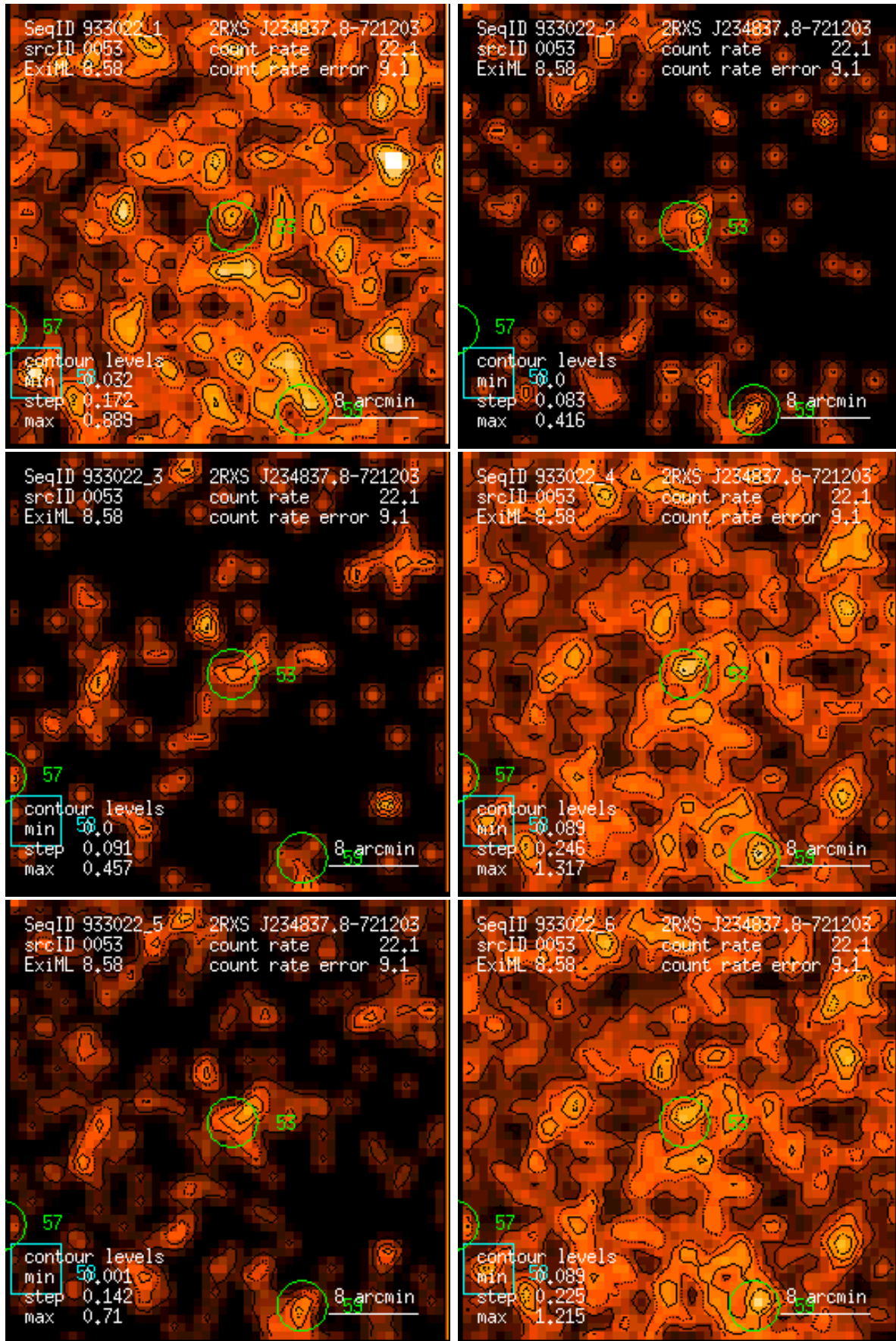
Figure 53: RASS 933022: detection 0053: band rate images, Gaussian filter: (1) PSPC channels 11 – 41, (2) 52 – 90, (3) 91 – 201, (4) 11 – 235, (5) 52 – 201, (6) 11 – 201. Broad band rates in counts/ks. Band rate contour levels in counts/ks/arcmin 2 .
