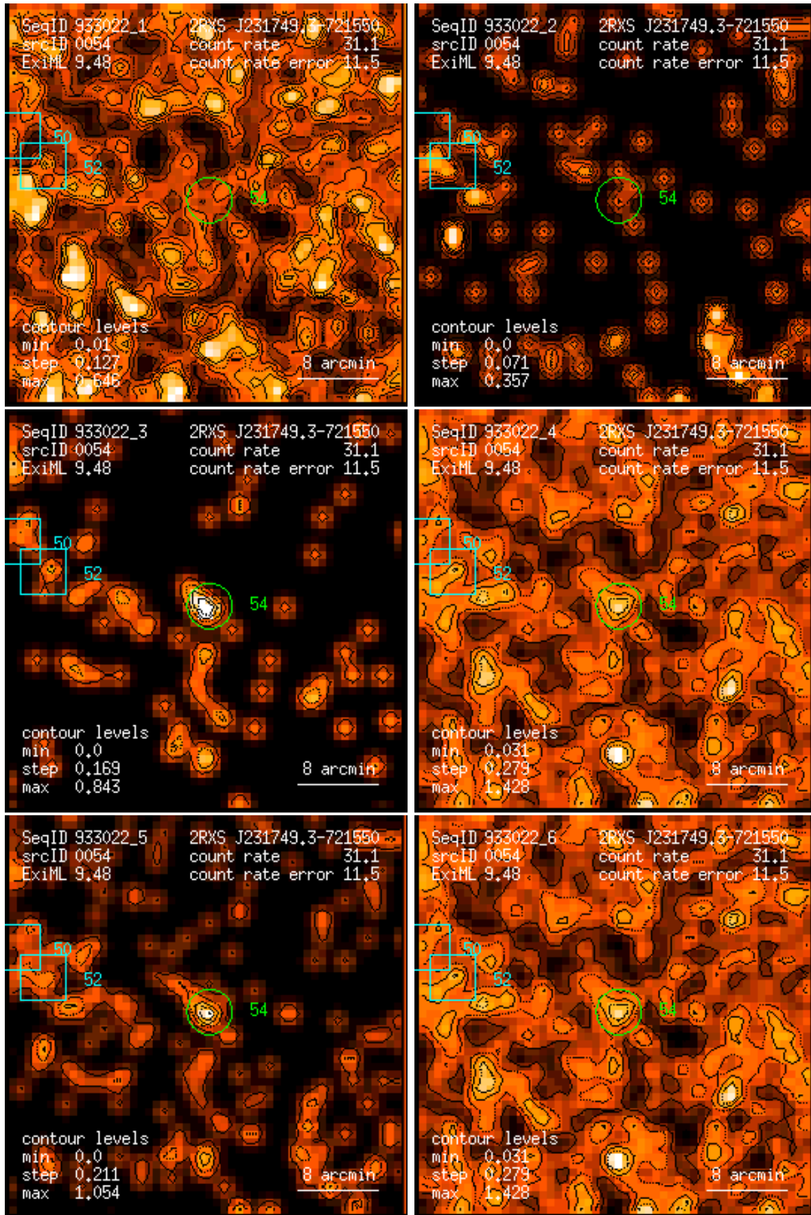
Figure 54: RASS 933022: detection 0054: band rate images, Gaussian filter: (1) PSPC channels 11 – 41, (2) 52 – 90, (3) 91 – 201, (4) 11 – 235, (5) 52 – 201, (6) 11 – 201. Broad band rates in counts/ks. Band rate contour levels in counts/ks/arcmin 2 .
