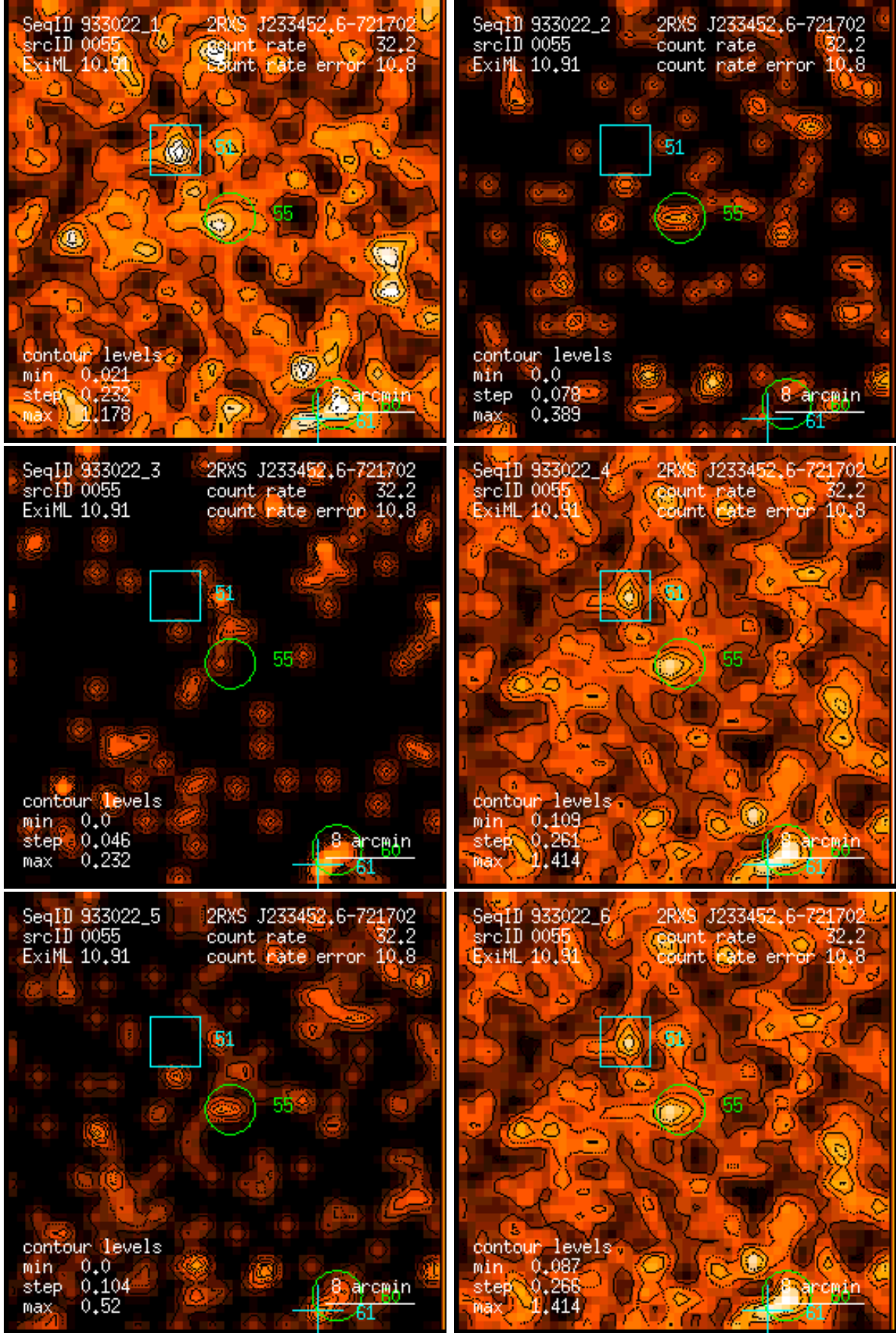
Figure 55: RASS 933022: detection 0055: band rate images, Gaussian filter: (1) PSPC channels 11 – 41, (2) 52 – 90, (3) 91 – 201, (4) 11 – 235, (5) 52 – 201, (6) 11 – 201. Broad band rates in counts/ks. Band rate contour levels in counts/ks/arcmin 2 .
