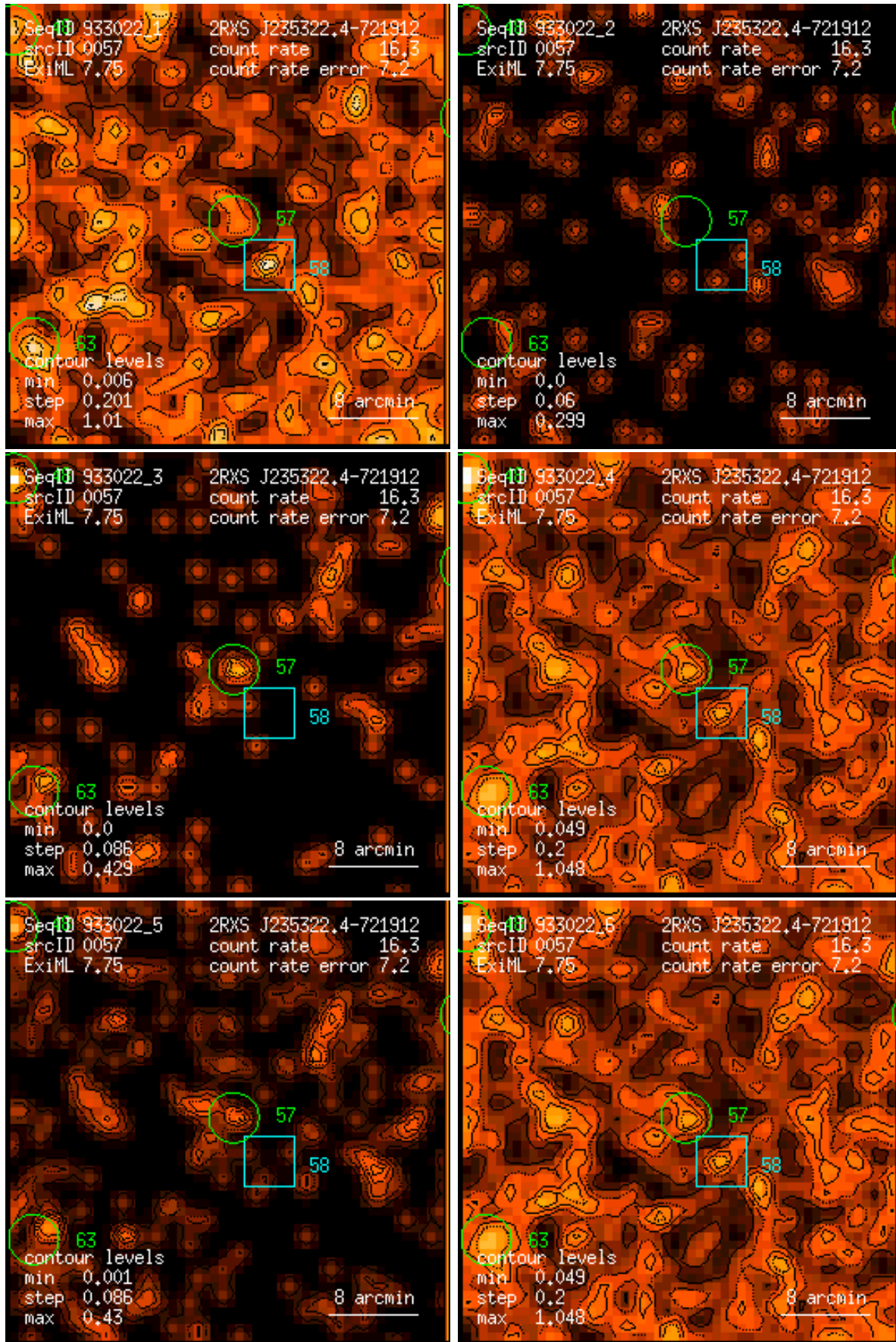
Figure 57: RASS 933022: detection 0057: band rate images, Gaussian filter: (1) PSPC channels 11 – 41, (2) 52 – 90, (3) 91 – 201, (4) 11 – 235, (5) 52 – 201, (6) 11 – 201. Broad band rates in counts/ks. Band rate contour levels in counts/ks/arcmin 2 .
