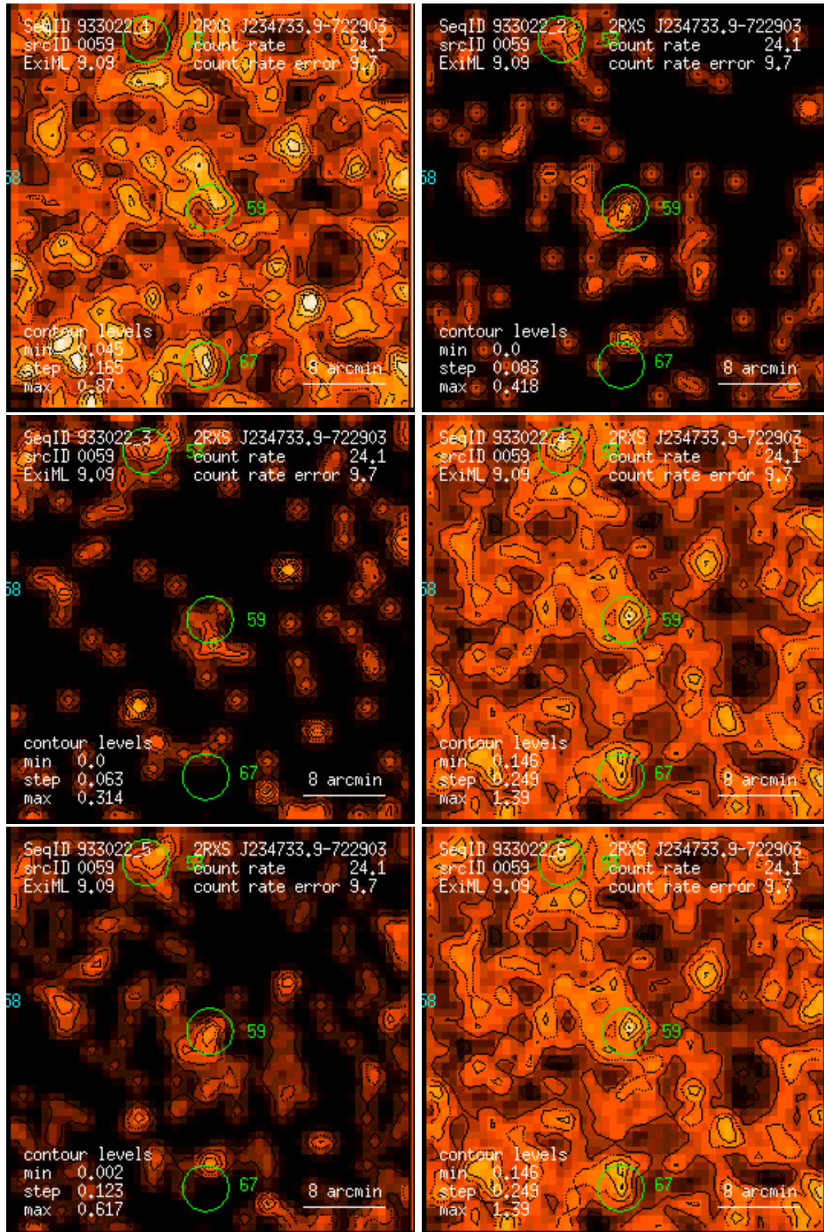
Figure 59: RASS 933022: detection 0059: band rate images, Gaussian filter: (1) PSPC channels 11 – 41, (2) 52 – 90, (3) 91 – 201, (4) 11 – 235, (5) 52 – 201, (6) 11 – 201. Broad band rates in counts/ks. Band rate contour levels in counts/ks/arcmin 2 .
