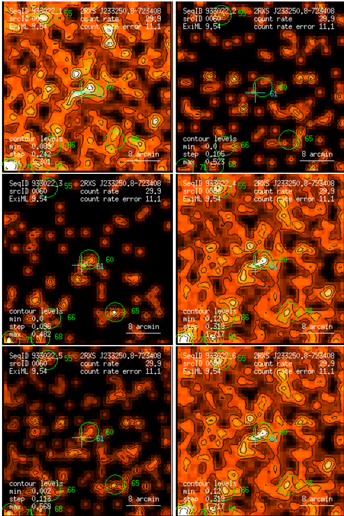
Figure 60: RASS 933022: detection 0060: band rate images, Gaussian filter: (1) PSPC channels 11 – 41, (2) 52 – 90, (3) 91 – 201, (4) 11 – 235, (5) 52 – 201, (6) 11 – 201. Broad band rates in counts/ks. Band rate contour levels in counts/ks/arcmin 2 .
