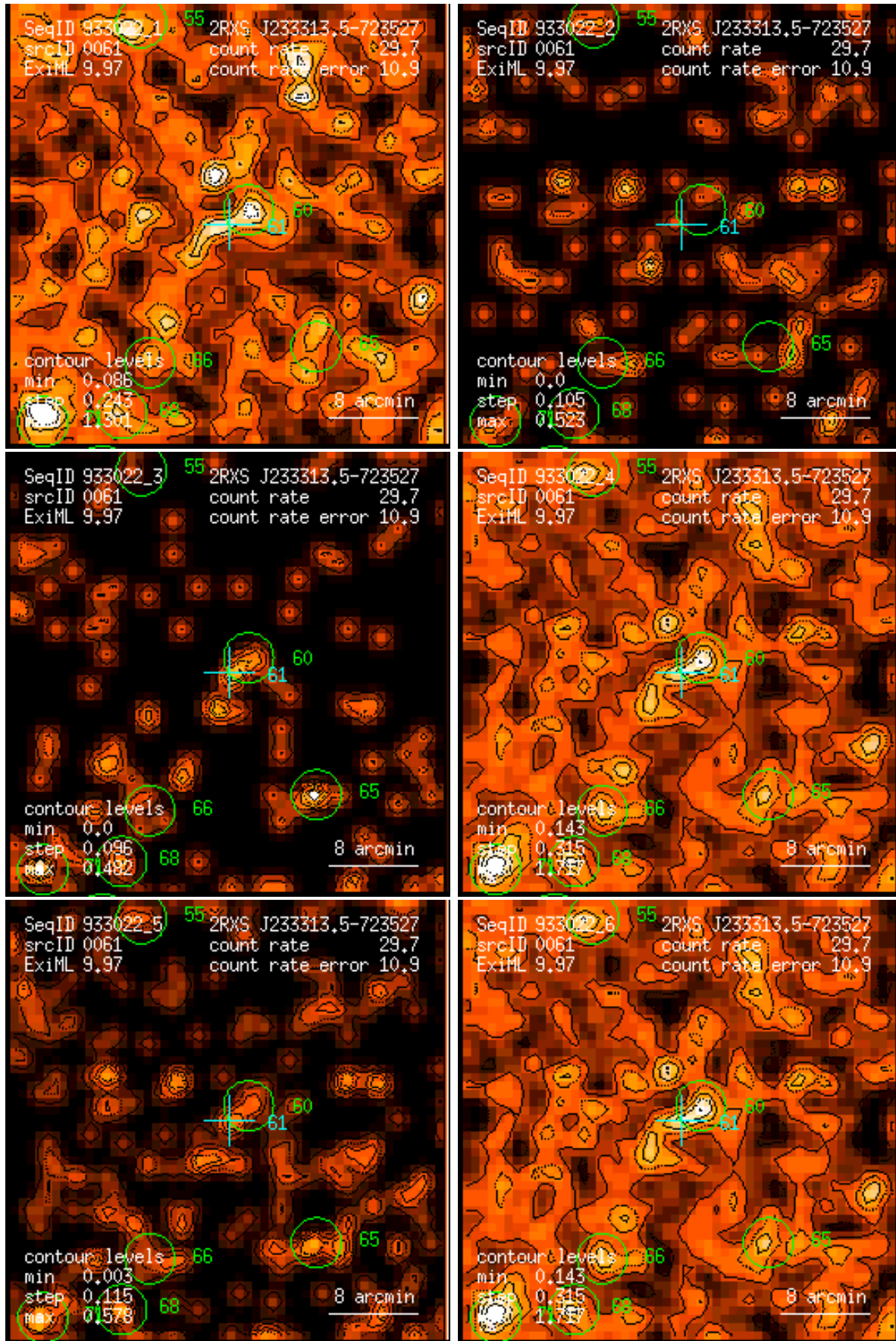
Figure 61: RASS 933022: detection 0061: band rate images, Gaussian filter: (1) PSPC channels 11 – 41, (2) 52 – 90, (3) 91 – 201, (4) 11 – 235, (5) 52 – 201, (6) 11 – 201. Broad band rates in counts/ks. Band rate contour levels in counts/ks/arcmin 2 .
