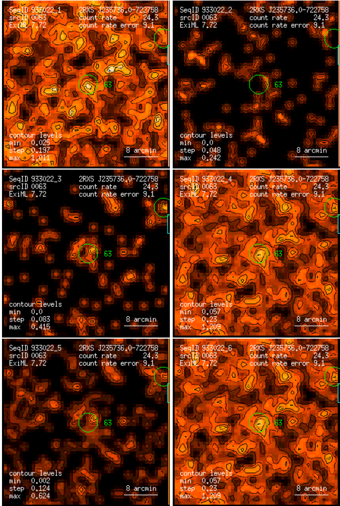
Figure 63: RASS 933022: detection 0063: band rate images, Gaussian filter: (1) PSPC channels 11 – 41, (2) 52 – 90, (3) 91 – 201, (4) 11 – 235, (5) 52 – 201, (6) 11 – 201. Broad band rates in counts/ks. Band rate contour levels in counts/ks/arcmin 2 .
