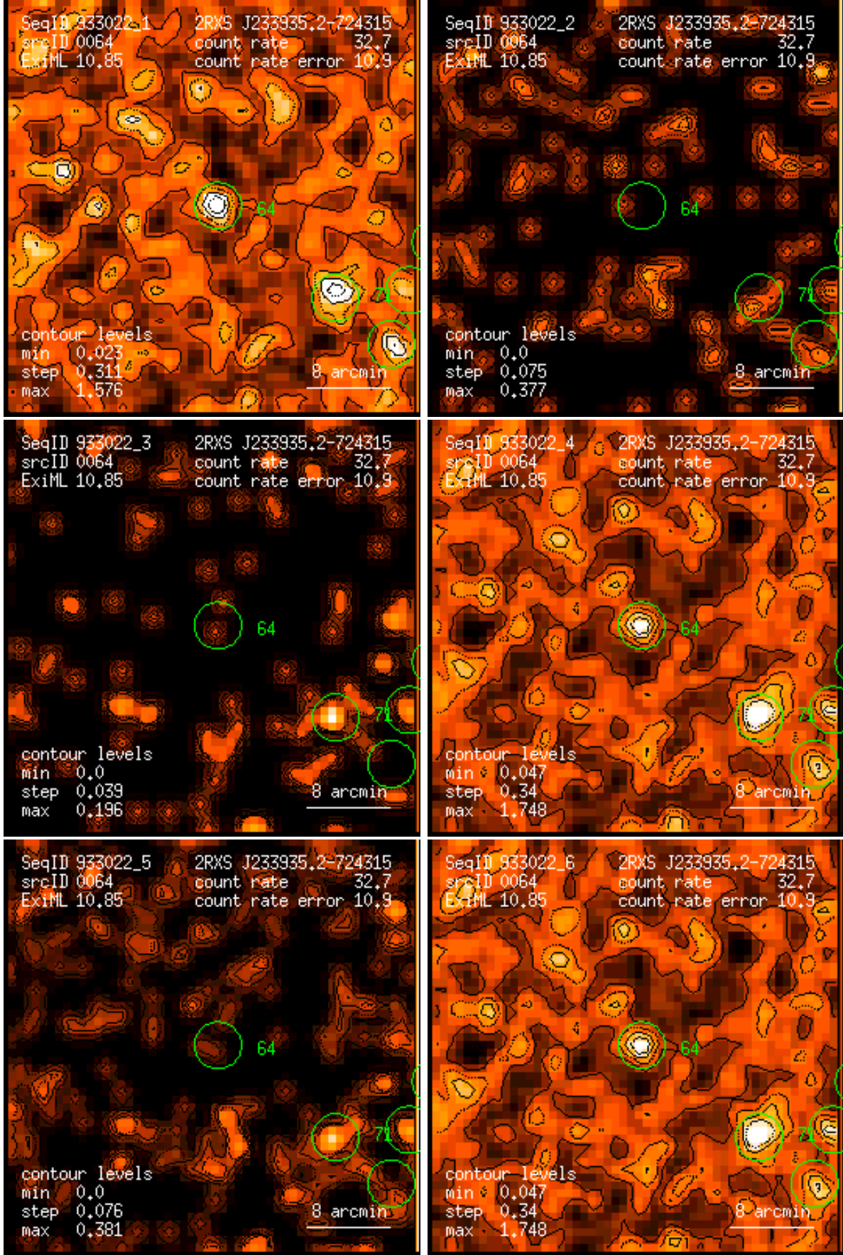
Figure 64: RASS 933022: detection 0064: band rate images, Gaussian filter: (1) PSPC channels 11 – 41, (2) 52 – 90, (3) 91 – 201, (4) 11 – 235, (5) 52 – 201, (6) 11 – 201. Broad band rates in counts/ks. Band rate contour levels in counts/ks/arcmin 2 .
